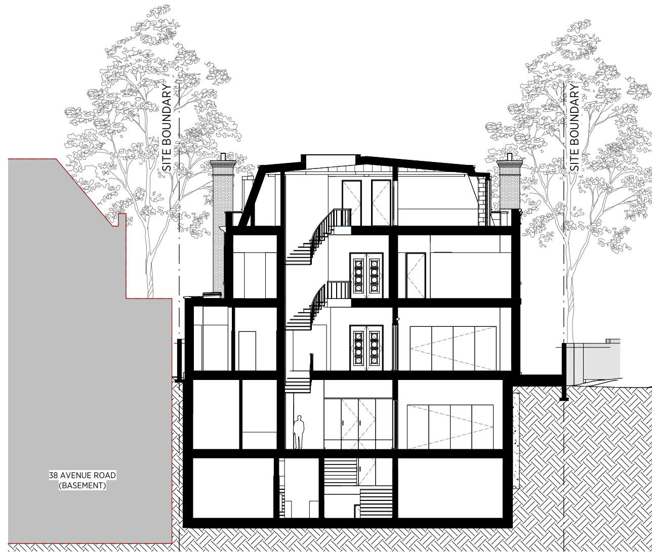
1 SECTION B-B 1:100
