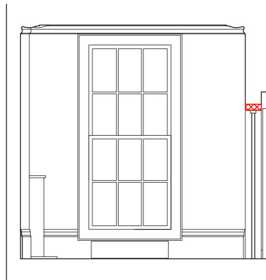
Section GG
