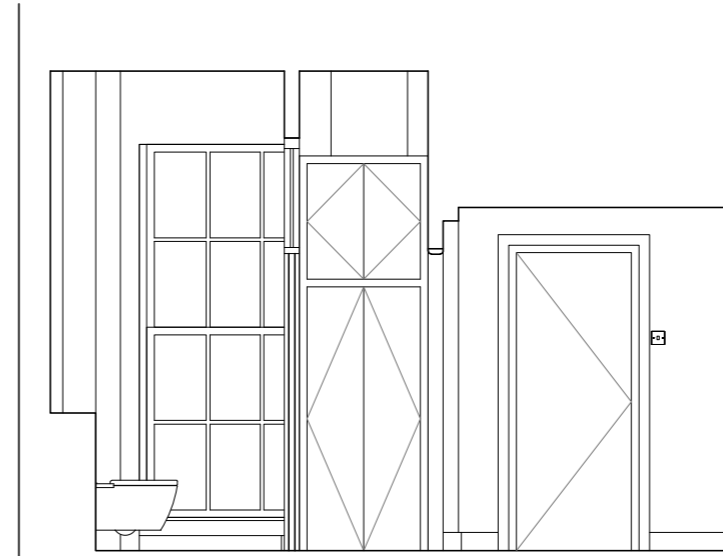
Section HH
