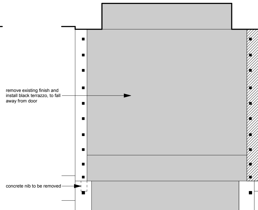
PROPOSED PLAN
