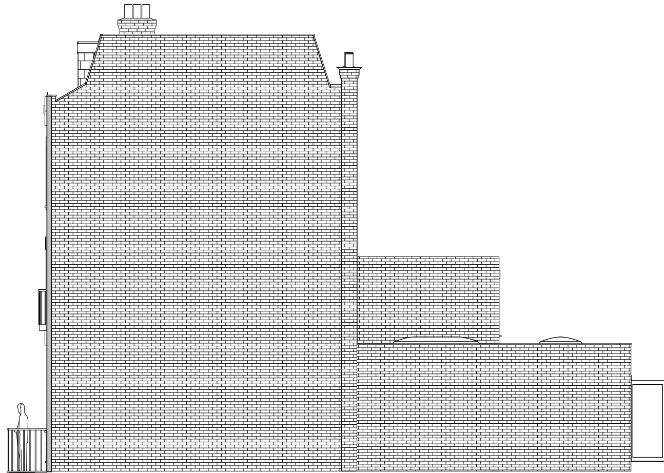
1 North Elevation 1 : 100
