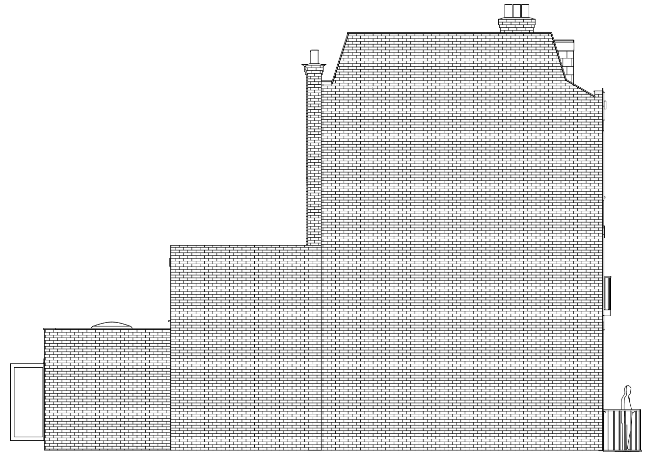
2 South Elevation 1 : 100
