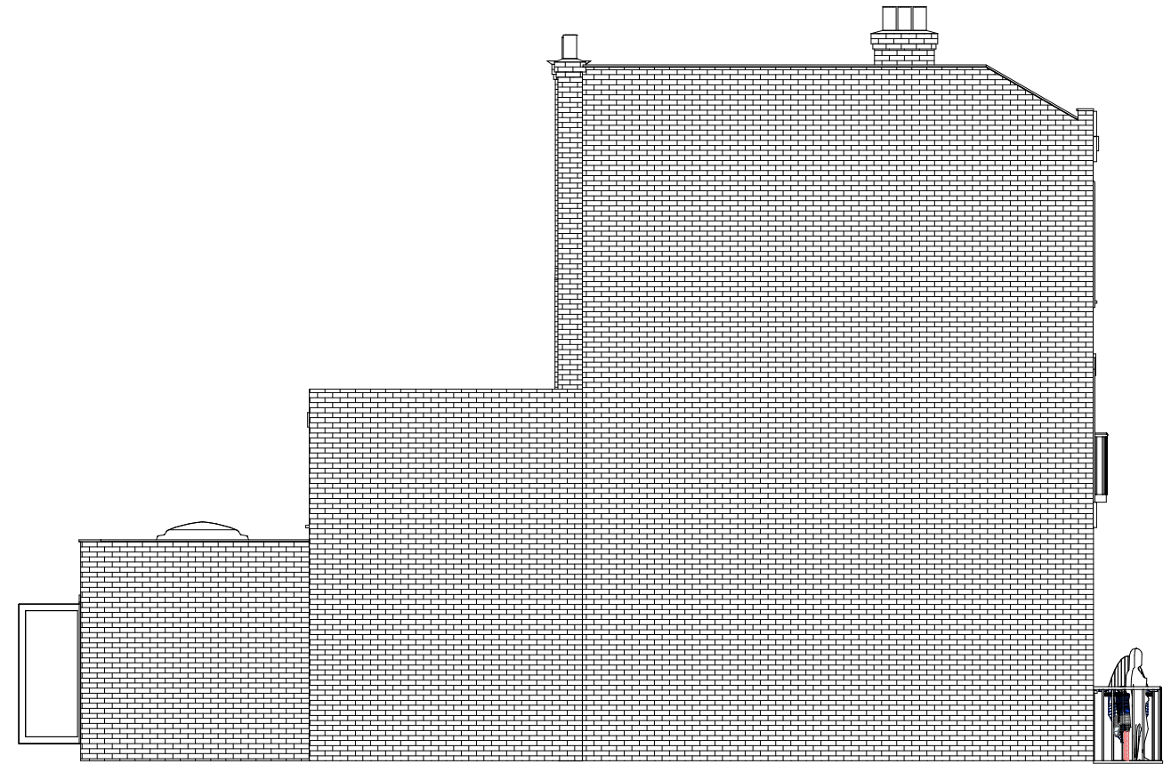
4 South Elevation 1 : 100
