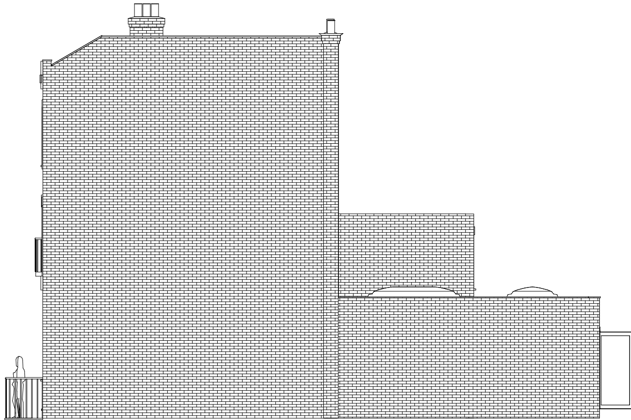
1 North Elevation 1 : 100
