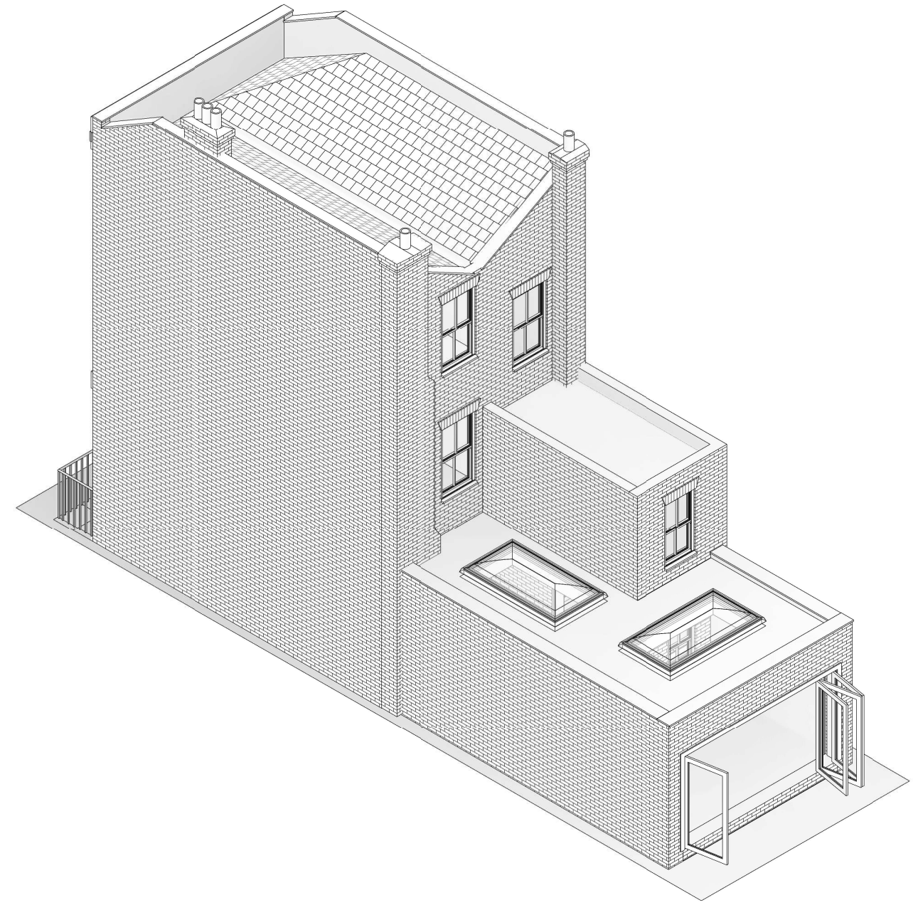
2 3d View 2-2
