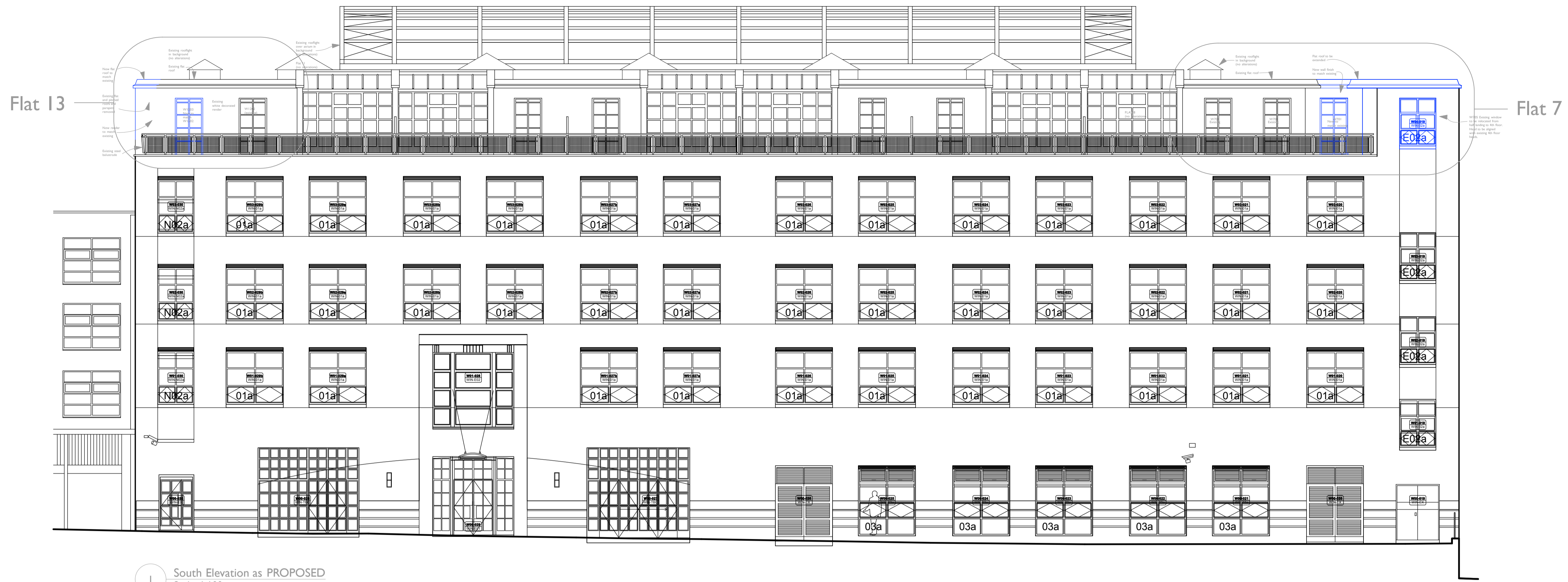
1 South Elevation as PROPOSED Scale: 1:100
