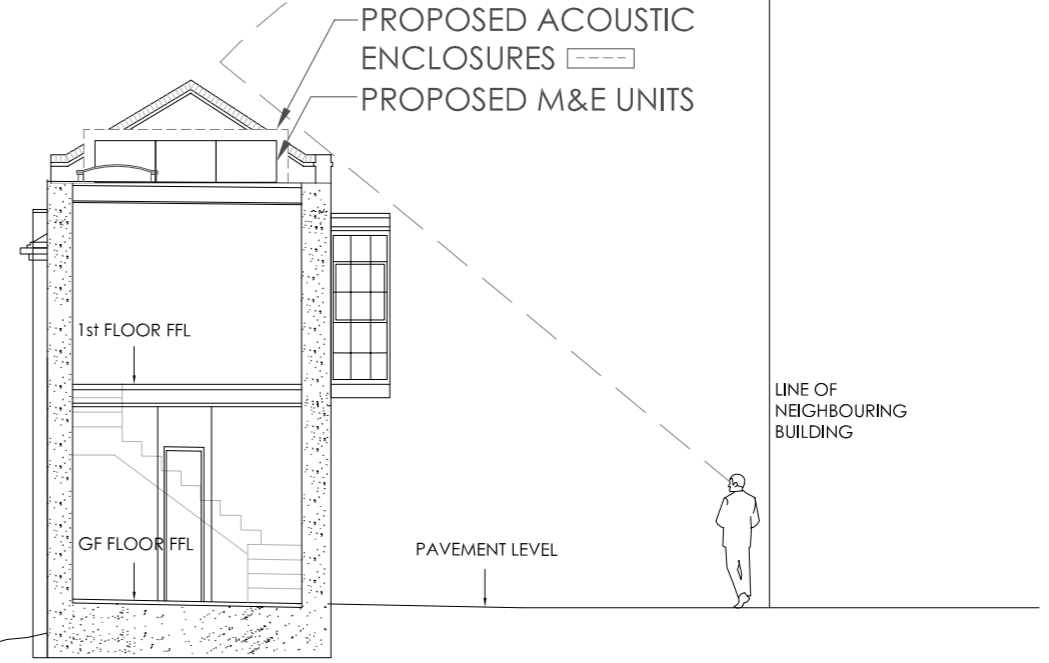
PROPOSED SECTION No 12A
