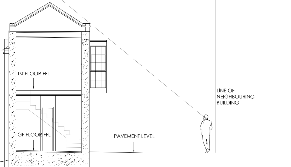
EXISTING SECTION No 12A
