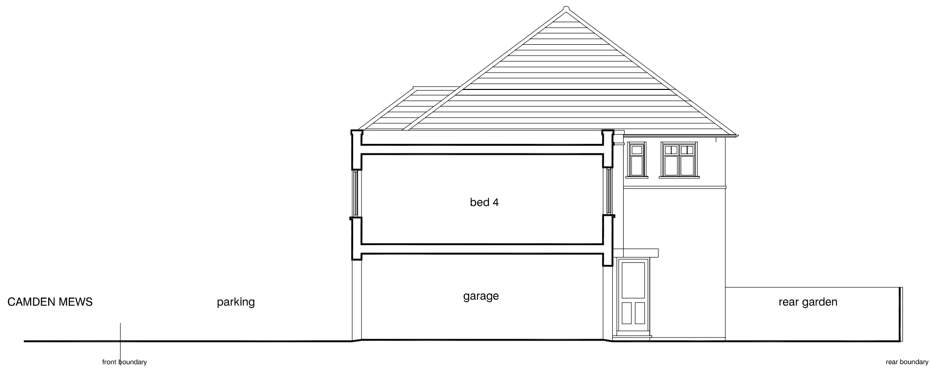
Sectional Elevation AA as existing
