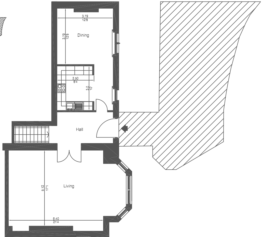
PLAN AT LOWER GROUND FLOOR LEVEL
