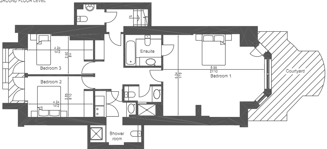
PLAN AT GROUND FLOOR LEVEL
