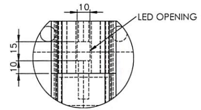
DETAIL L SCALE 1 : 2
