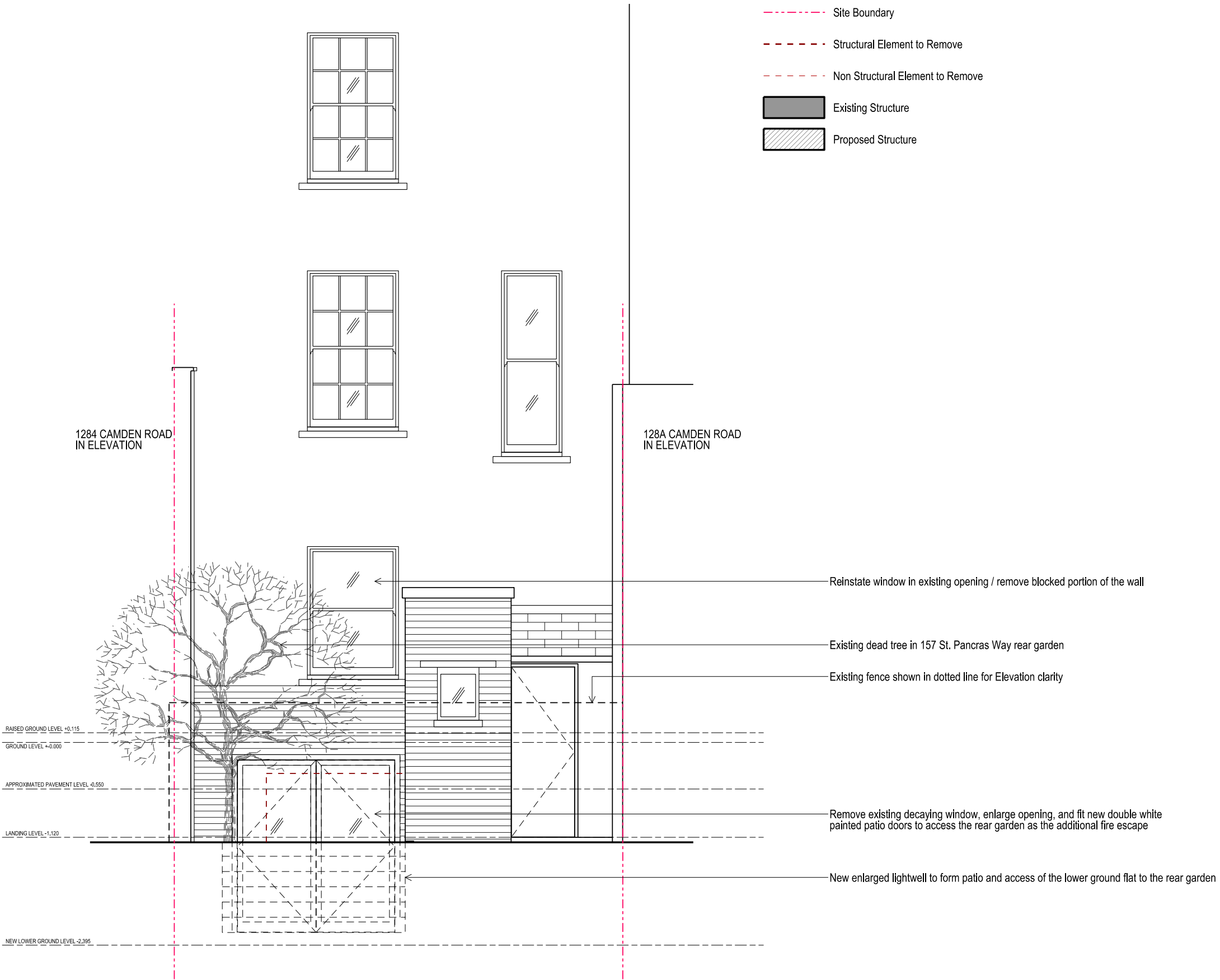
1 Proposed Rear Elevation Scale 1:50
