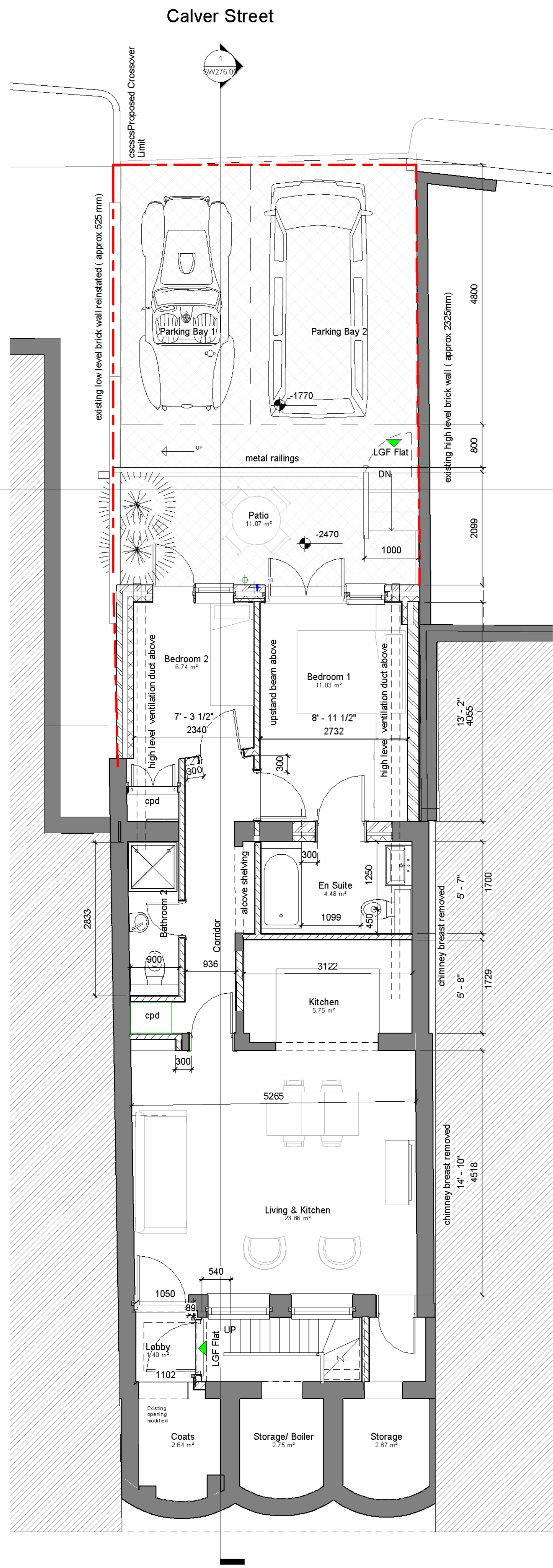
Proposed Lower Ground Floor Level. 1 : 50
