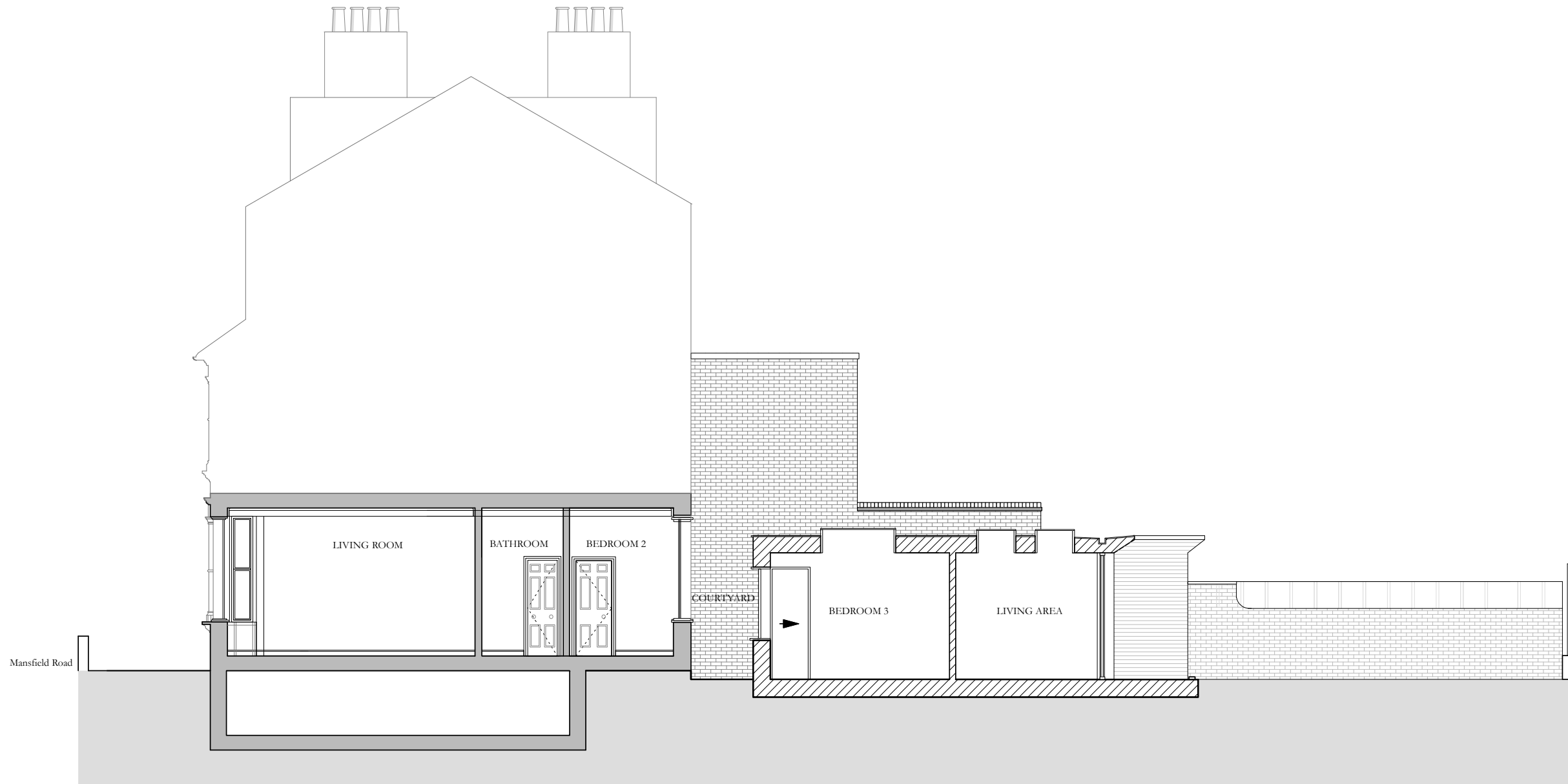
SECTION BB
