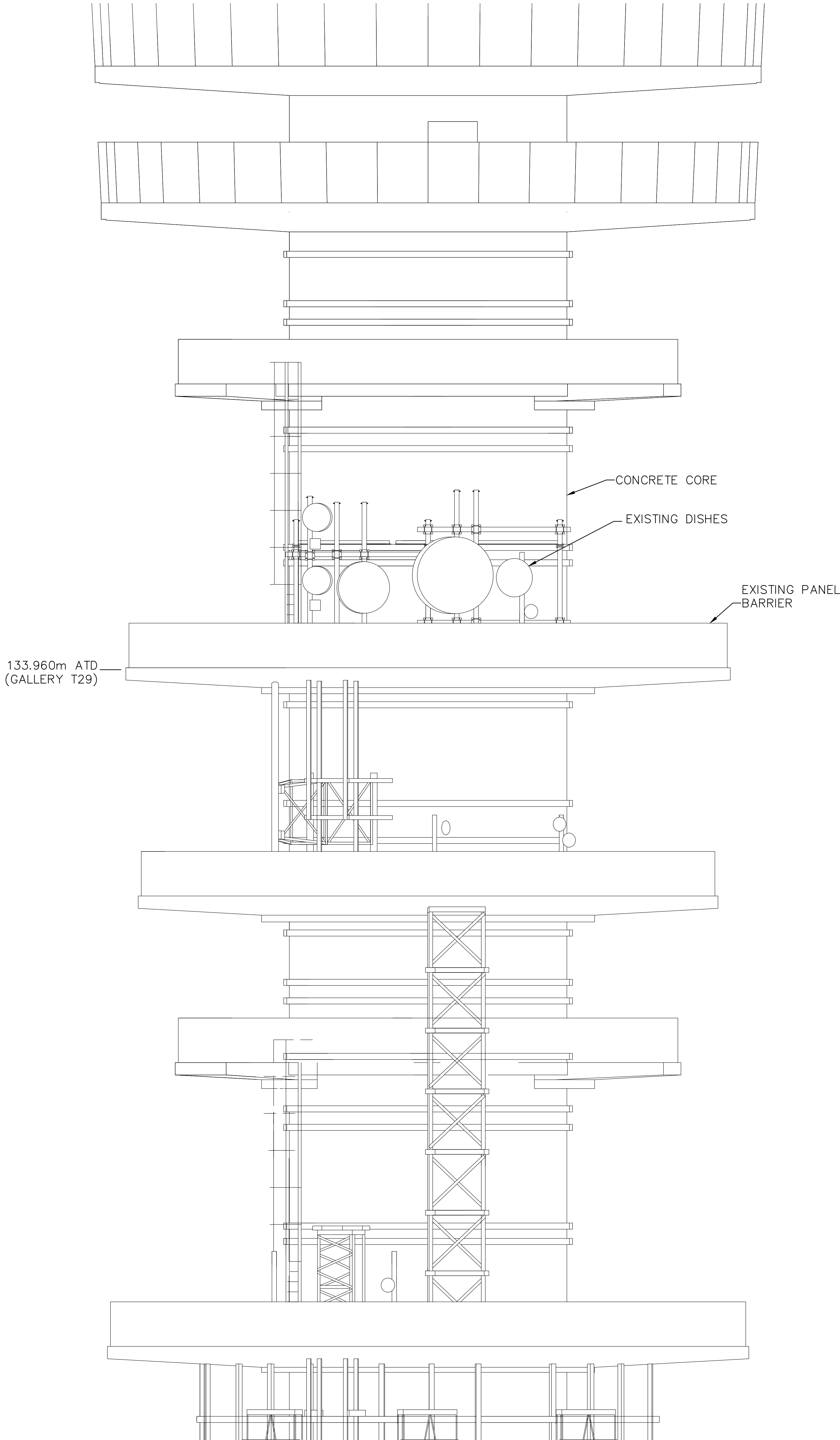
ENLARGED PART ELEVATION VIEW OF TOWER FACING WEST SHOWING EXISTING AERIALS SCALE 1:50
