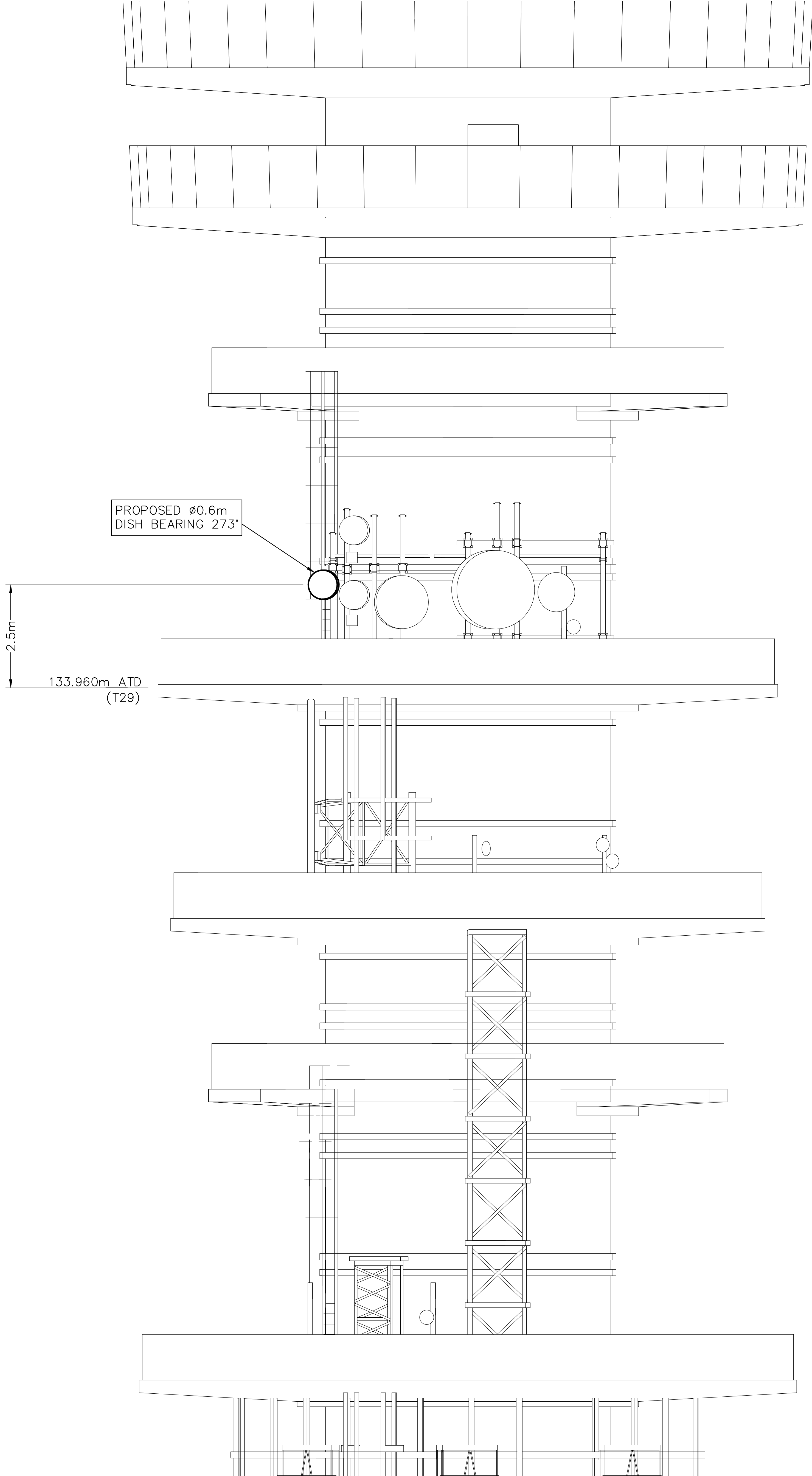
PART ELEVATION VIEW OF TOWER FACING WEST SHOWING PROPOSED AERIALS SCALE 1:50
