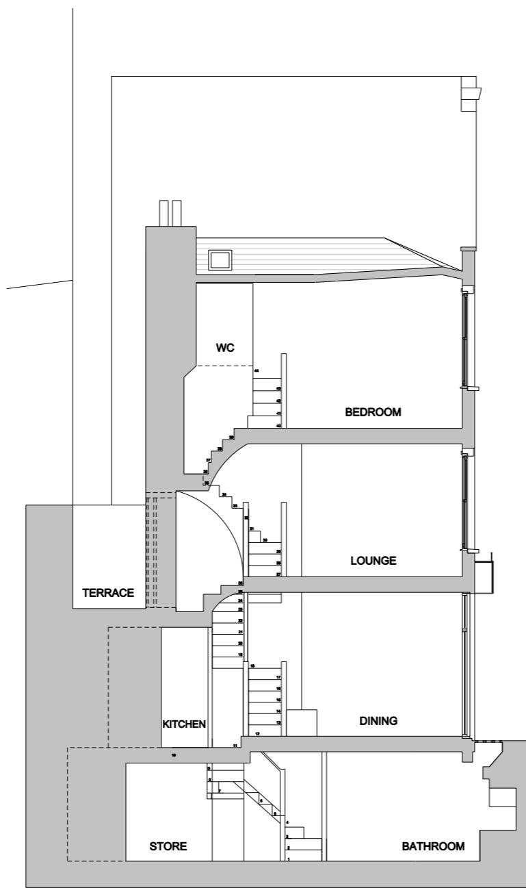
SECTION AA
