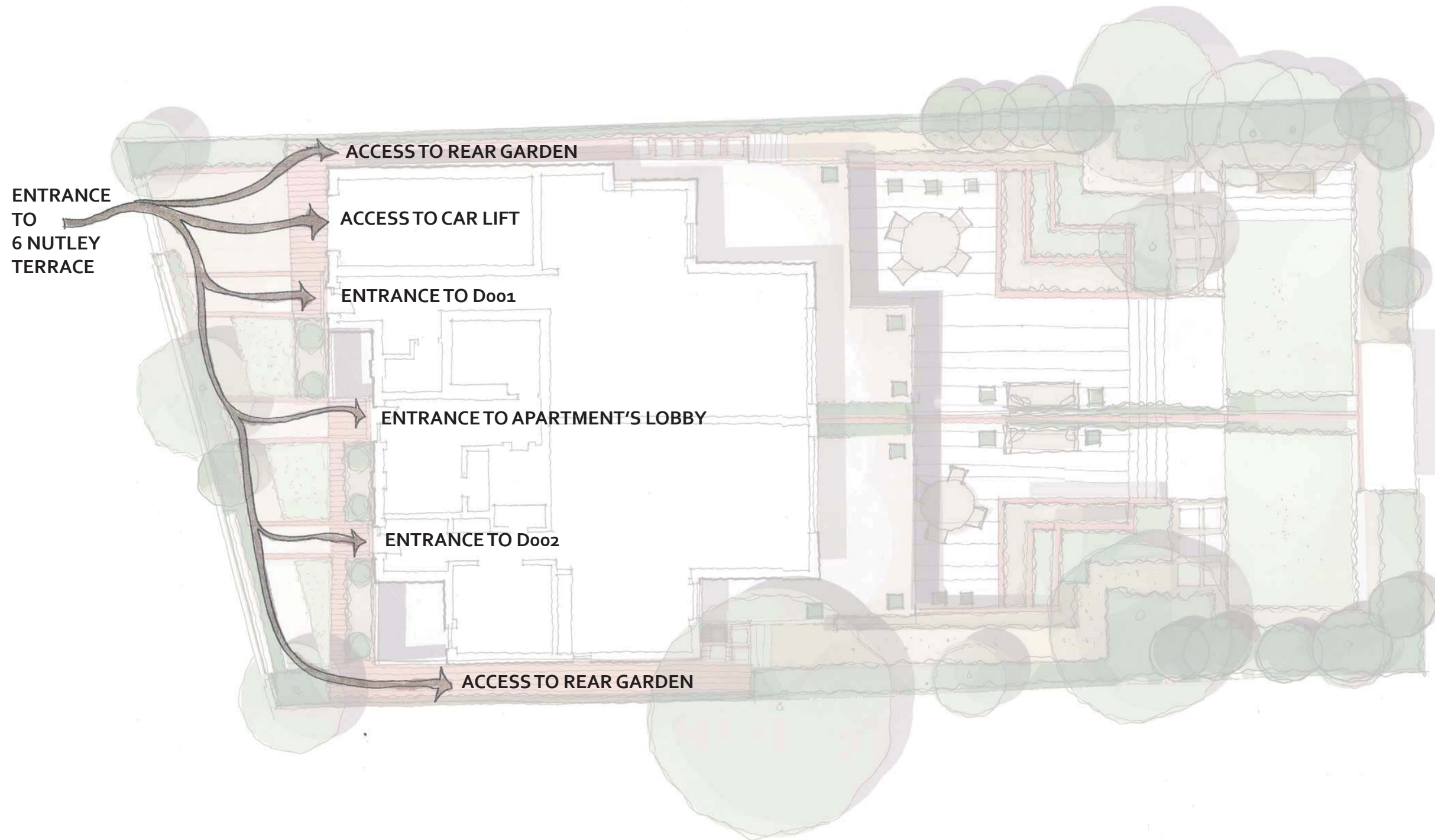
LANDSCAPE, FRONT GARDEN CIRCULATION PLAN
