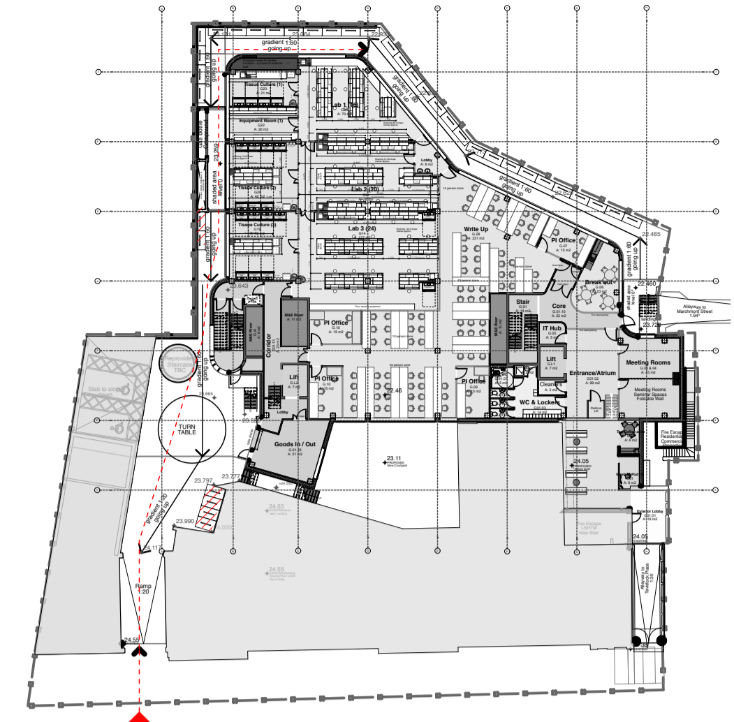
Proposed Cycle Entrance through the existing pend and route around the Proposed BRI Ground Floor Level Scale 1:500
