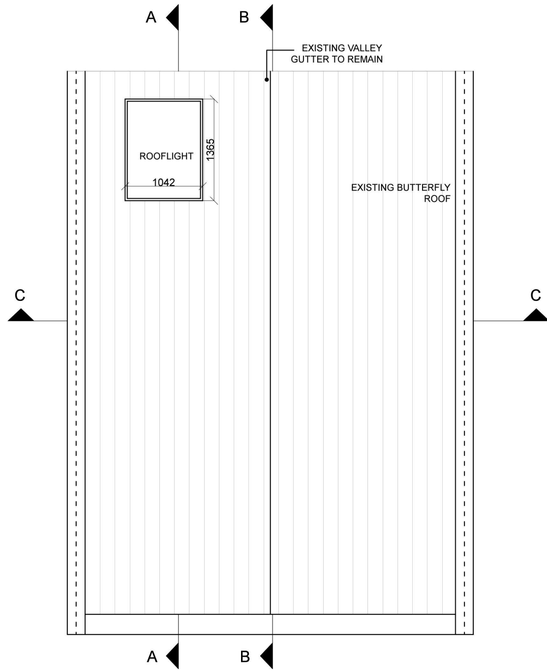
ROOF PLAN
