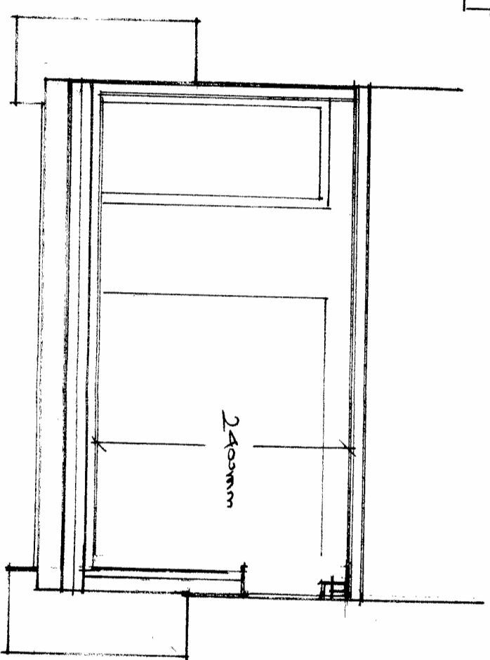
SECTION B-B
