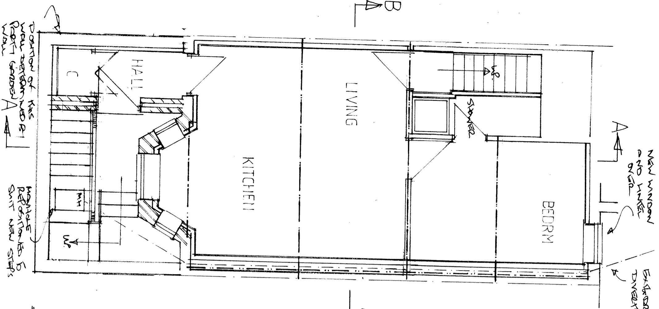
FLOOR PLAN
