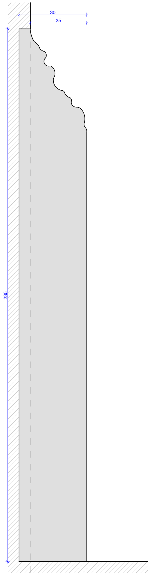
1:1 Skirting Profile
