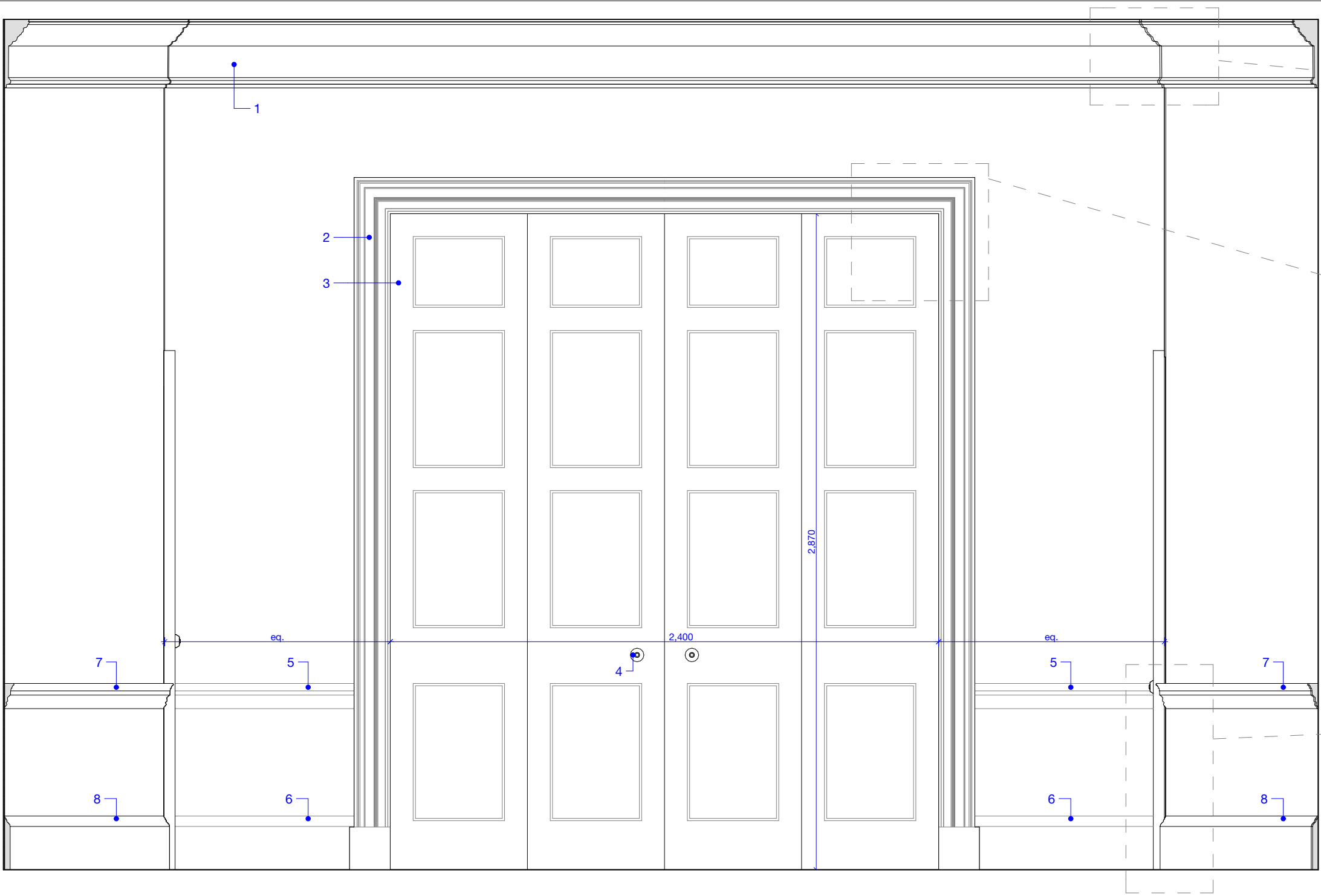
1:20 Proposed Ground Floor Door
