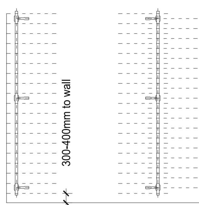
JOSTA STANDS EXAMPLE LAYOUT
