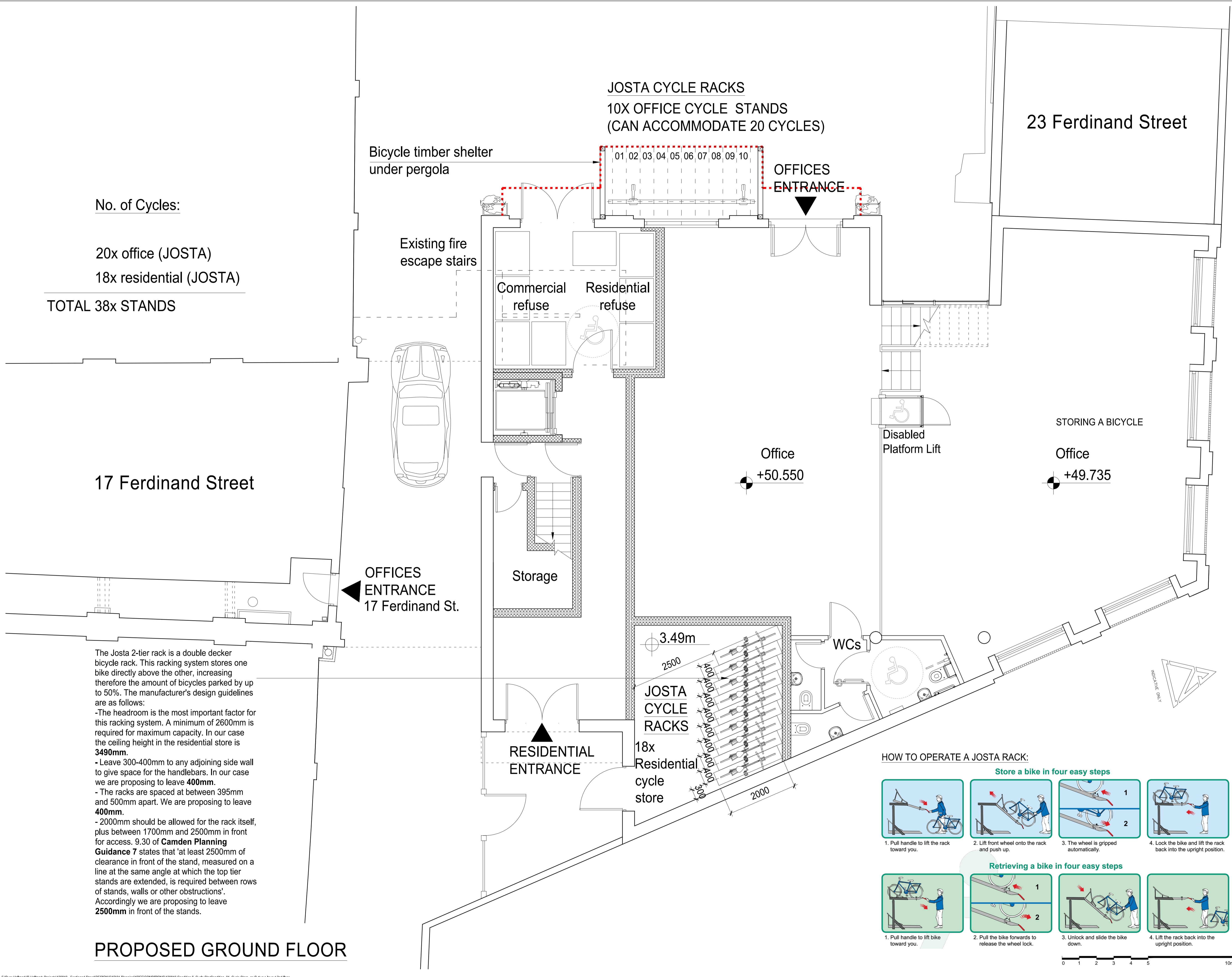
JOSTA STANDS EXAMPLE LAYOUT
