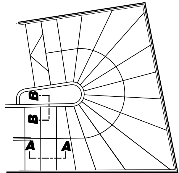
PRINCIPAL PLAN DIAGRAM STAIRCASE FIRST - SECOND FLOOR
