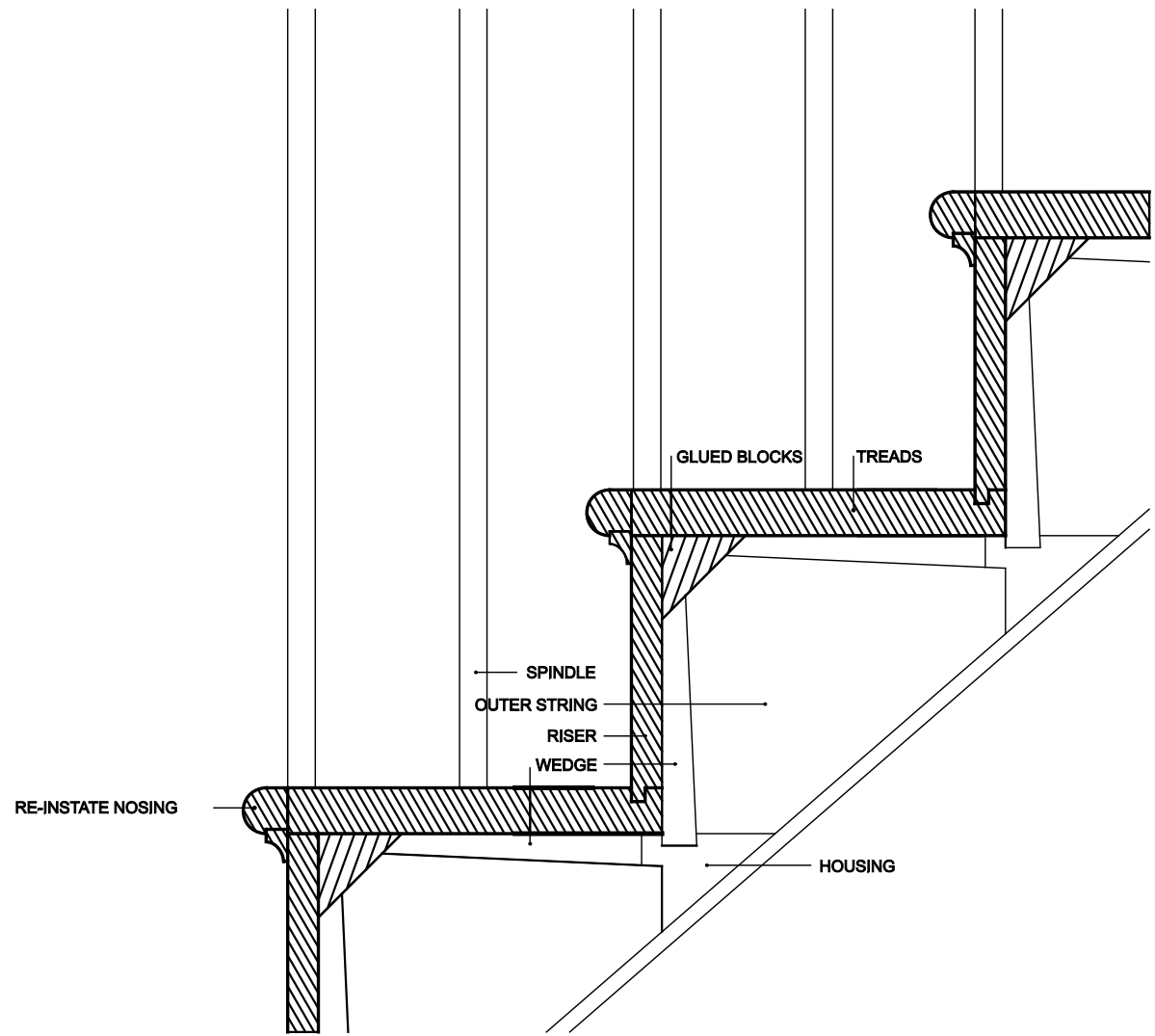
PRINCIPAL SECTION A-A 1:5
