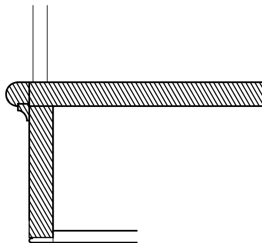
PRINCIPAL SECTION B-B 1:5
