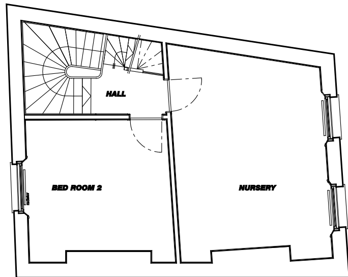
SECOND FLOOR PLAN 1:100 1968
