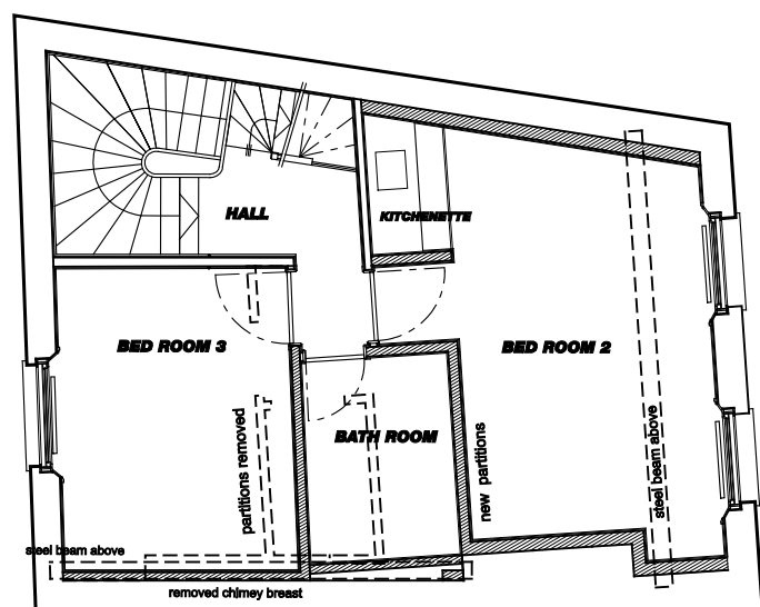
SECOND FLOOR PLAN 1:100 POST 2005
