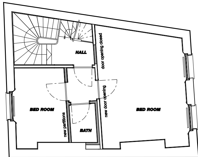
SECOND FLOOR PLAN 1:100 POST 1969
