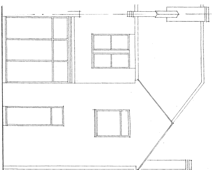
Rear Elevation
