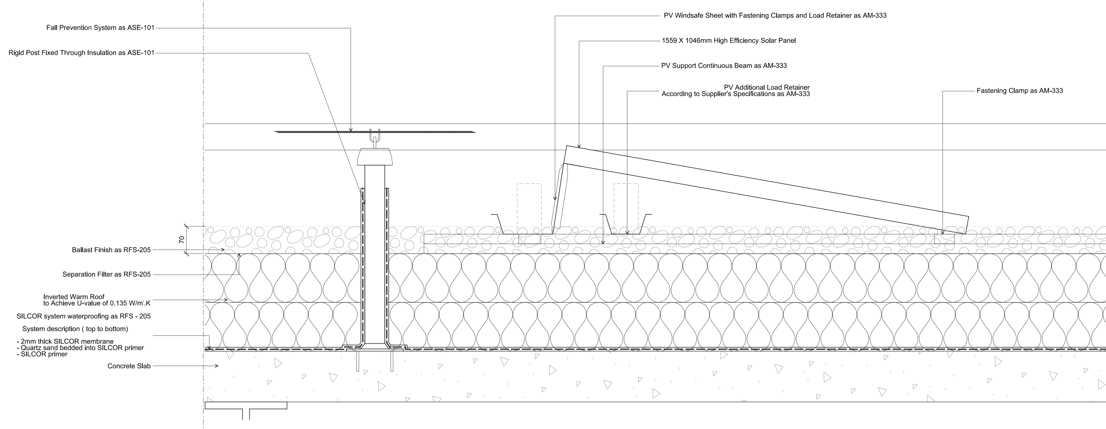
A SOLAR PANEL ON BALASTED ROOF Detail Section 1:5
