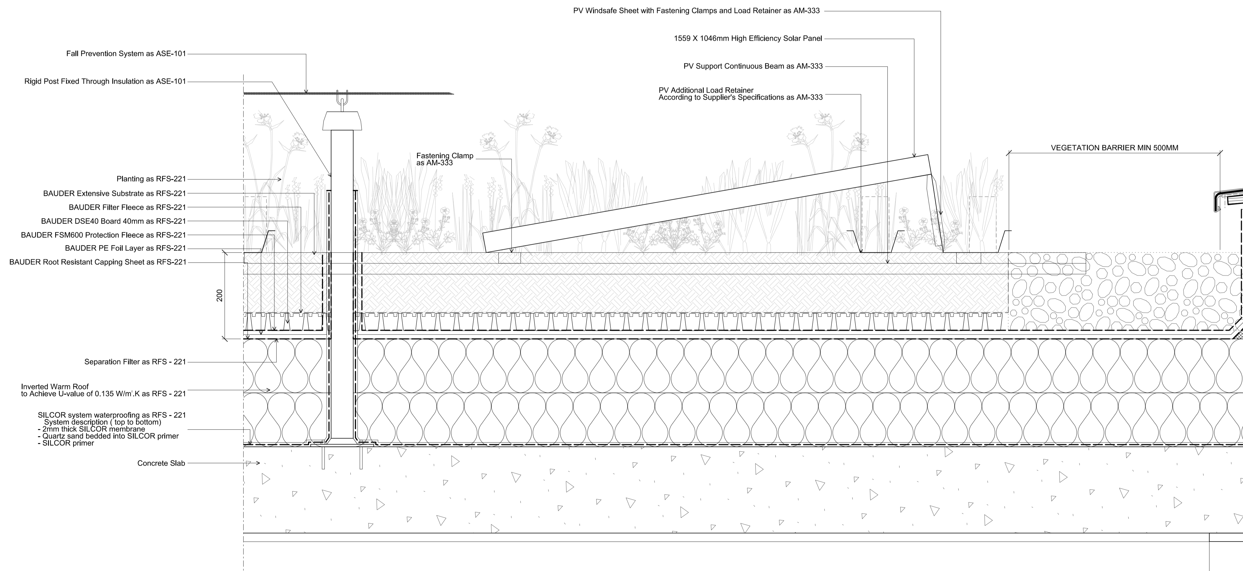
B SOLAR PANEL ON GREEN/BROWN ROOF Detail Section 1:5
