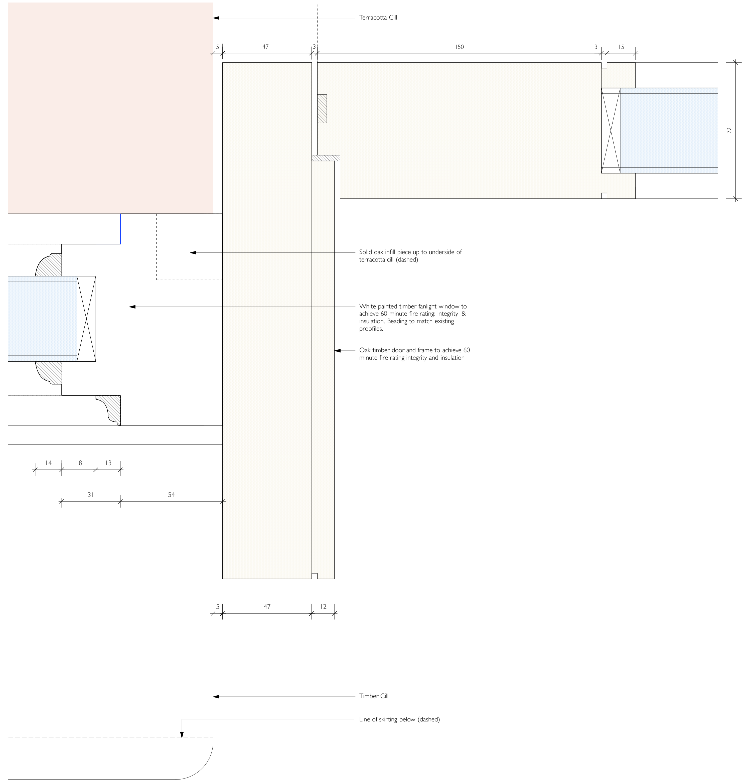
20 Proposed 60 Minute Fire Rated Door - Jamb Detail 1:1
