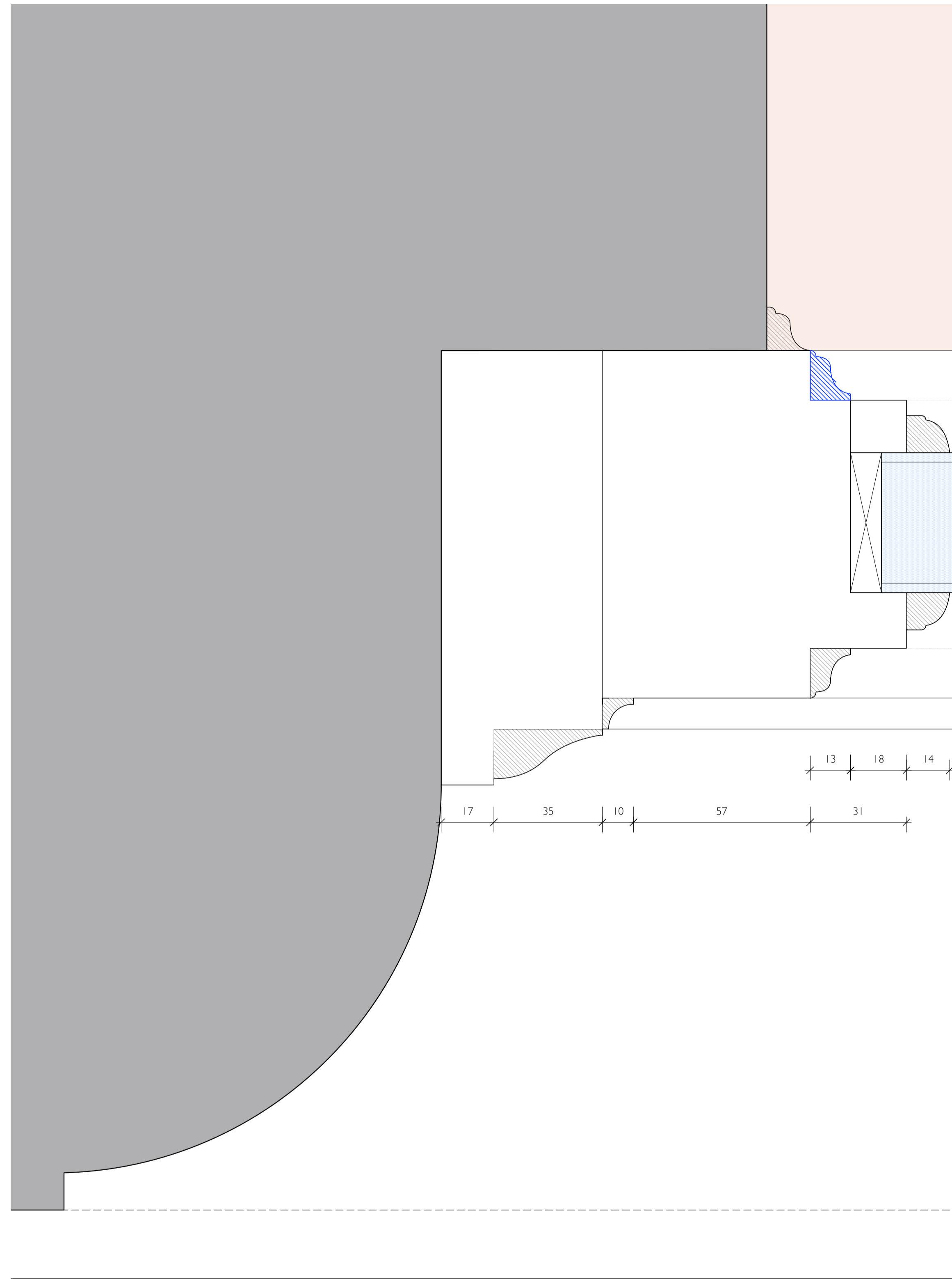
19 Proposed 60 Minute Fire Rated Door Fanlight - Jamb Detail 1:1
