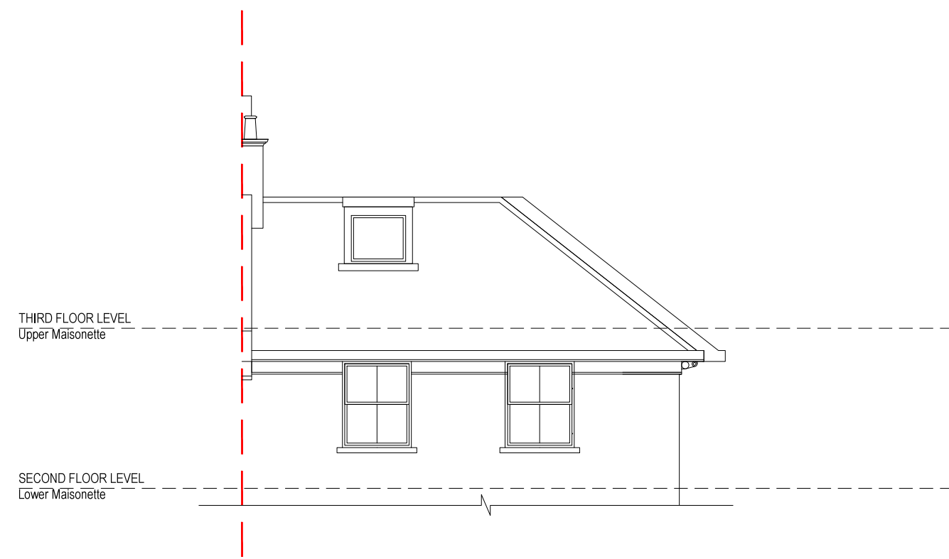
Existing - Rear Elevation (North East) SCALE : 1:100 @ A3
