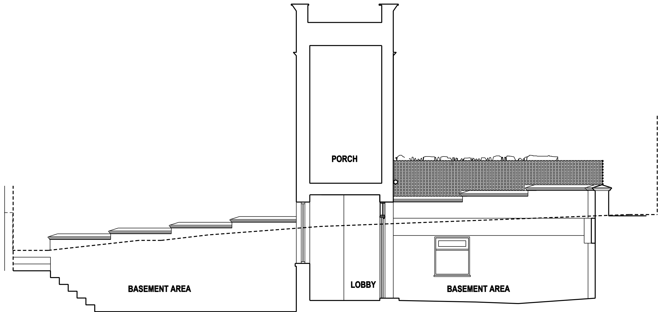
SECTION B
