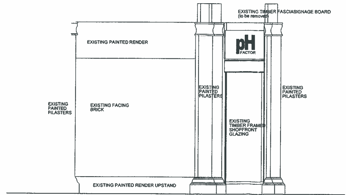
EXISTING PART ELEVATION BERKLEY ROAD
