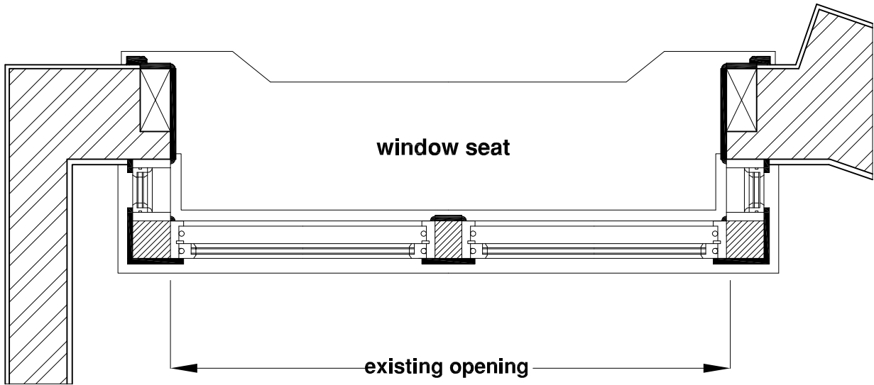
NEW GROUND FLOOR BAY WINDOW
