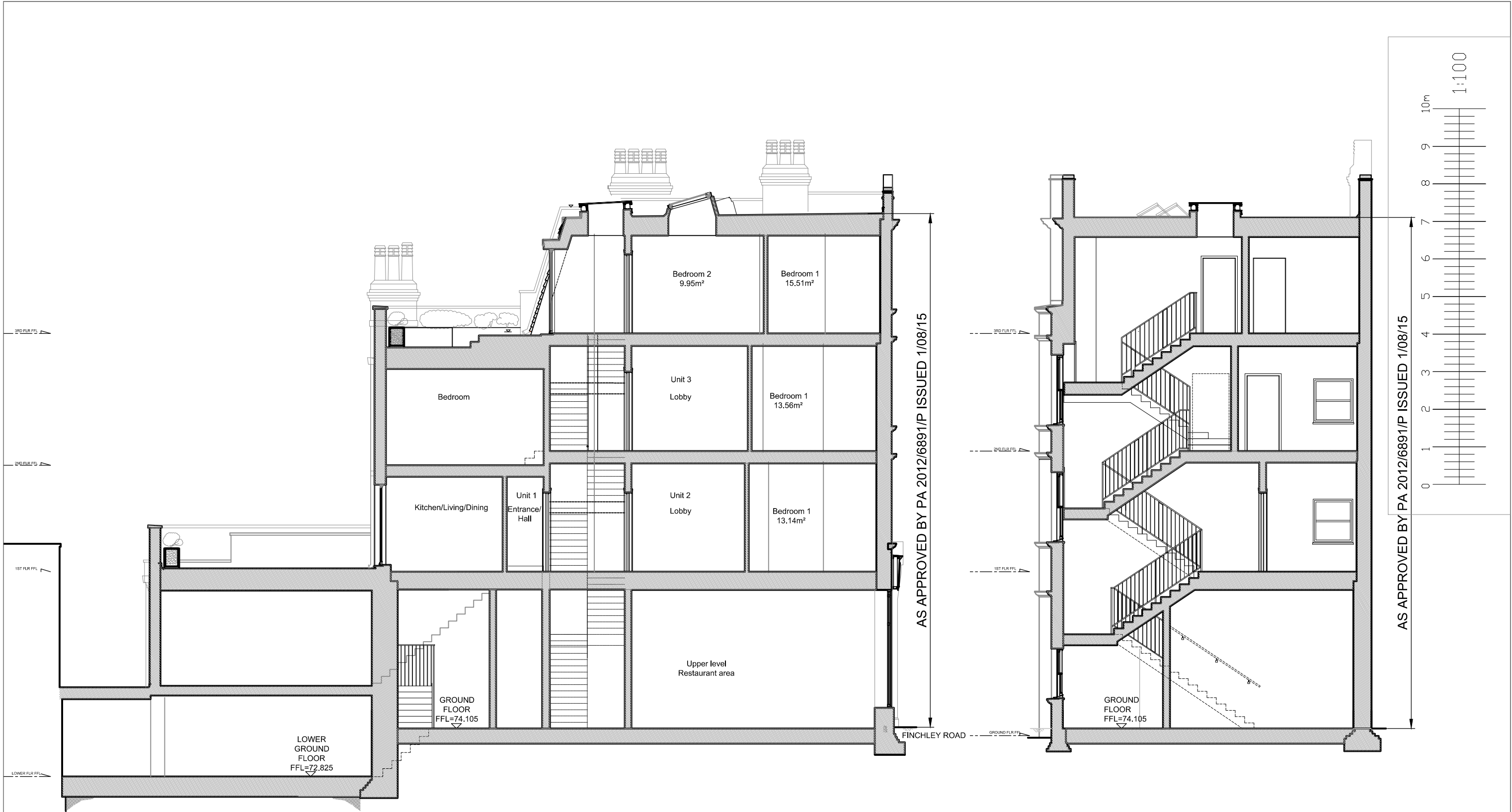
1 Existing Section A-A SCALE 1:100 @ A3
