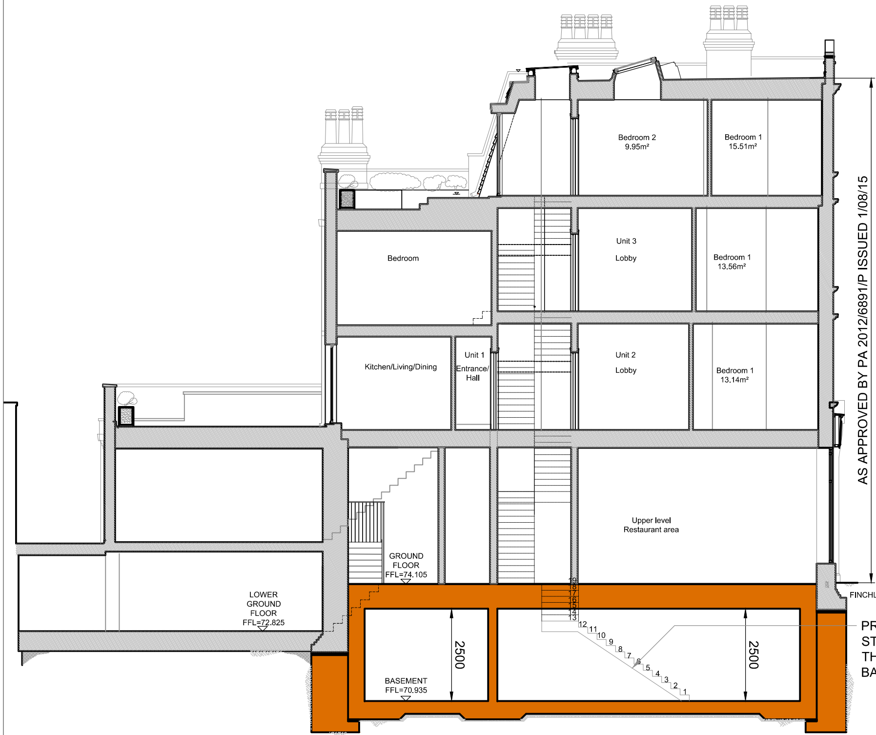
1 Proposed Section A-A 201 SCALE 1:100 @ A3
