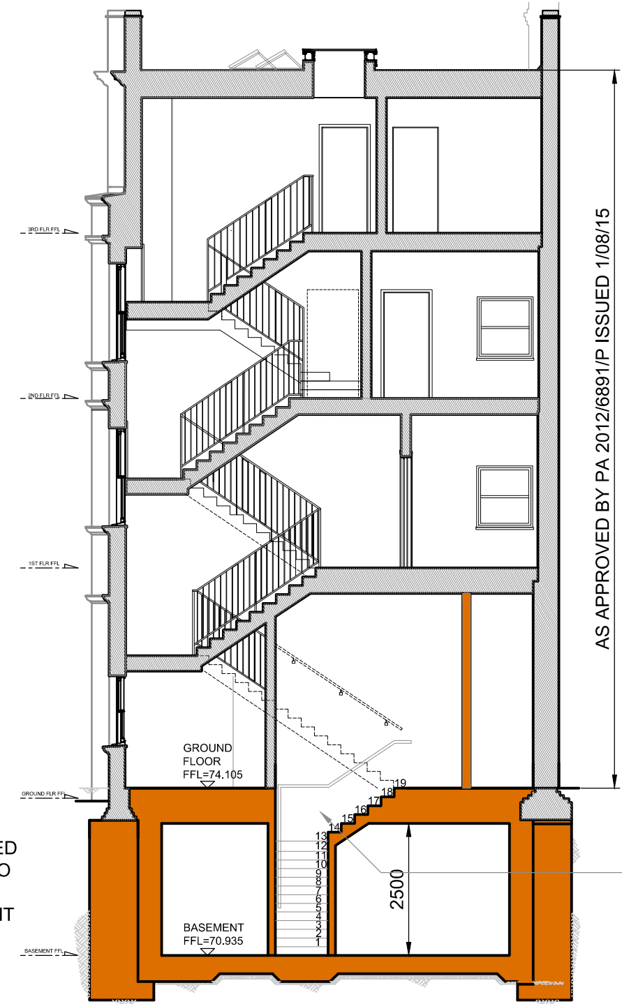
2 Proposed Section B-B 201 SCALE 1:100 @ A3
