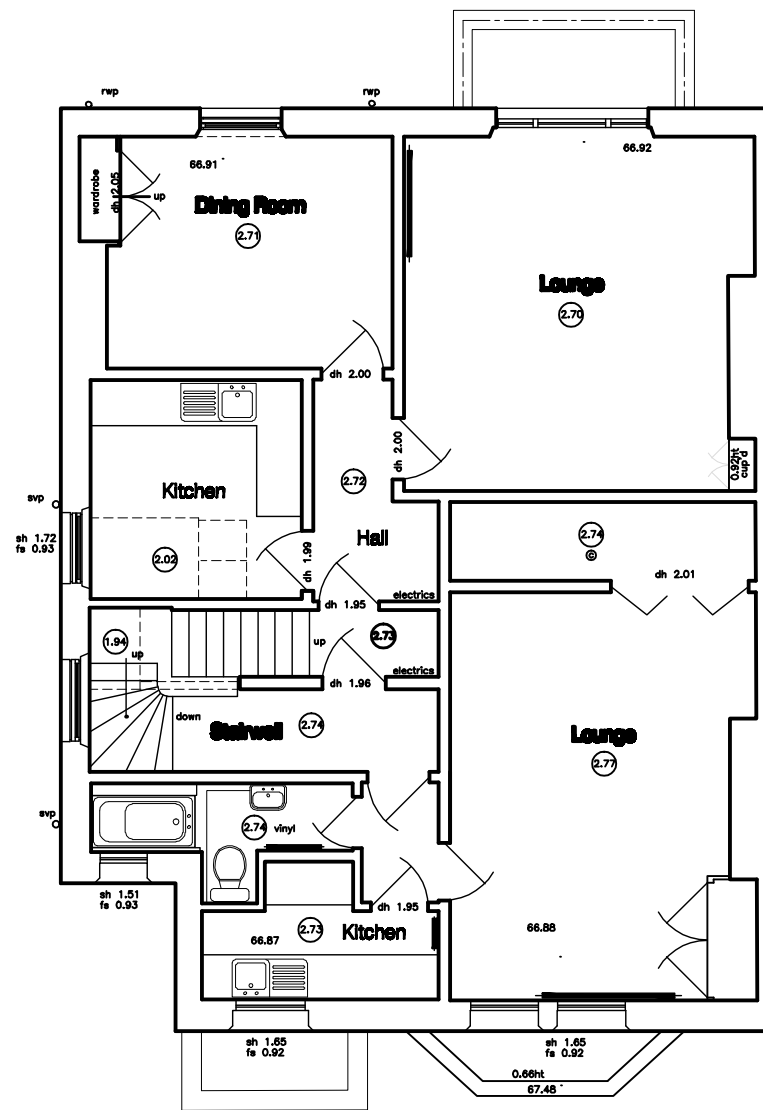
Second Floor Plan 1:100
