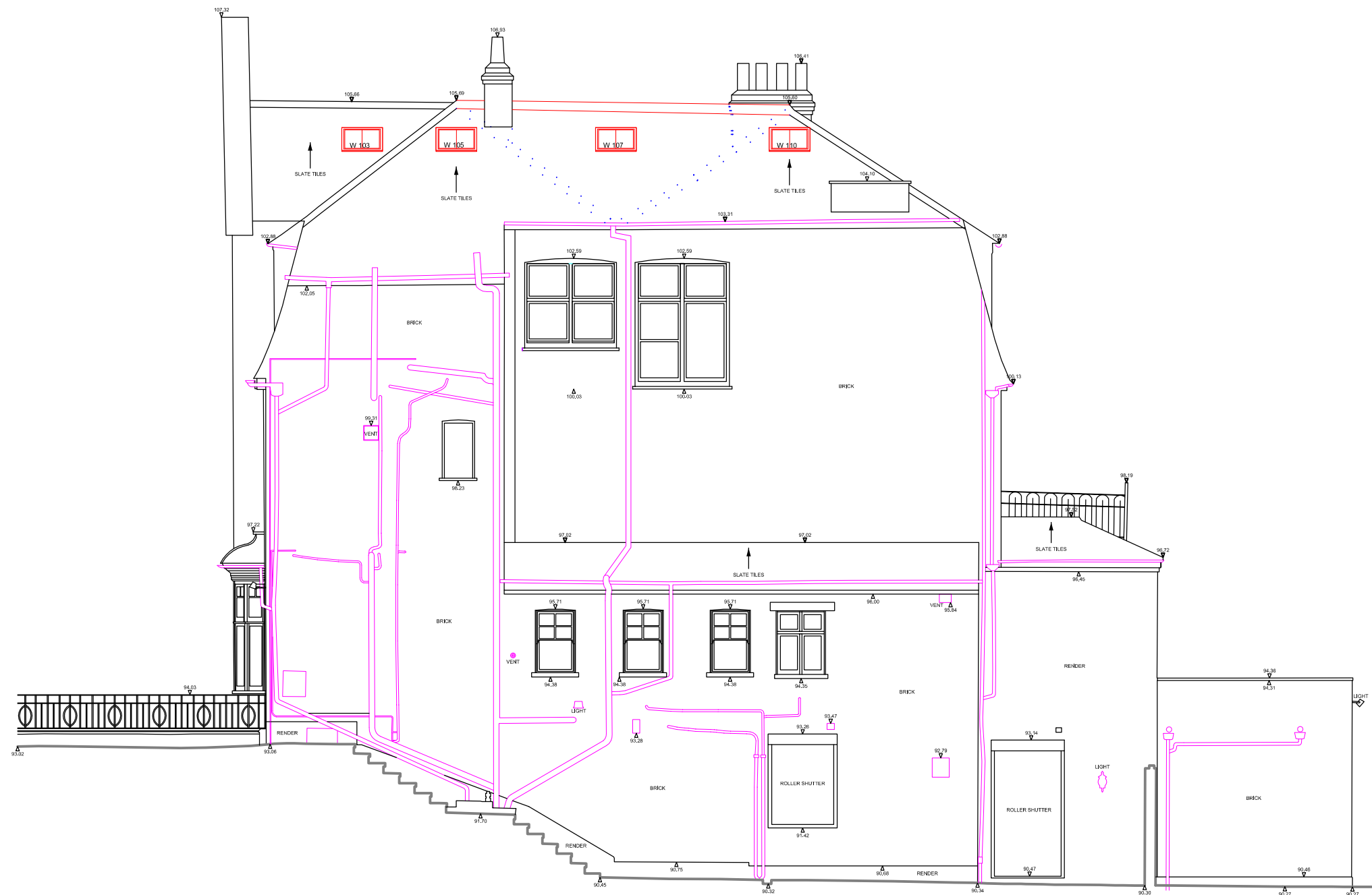
West elevation
