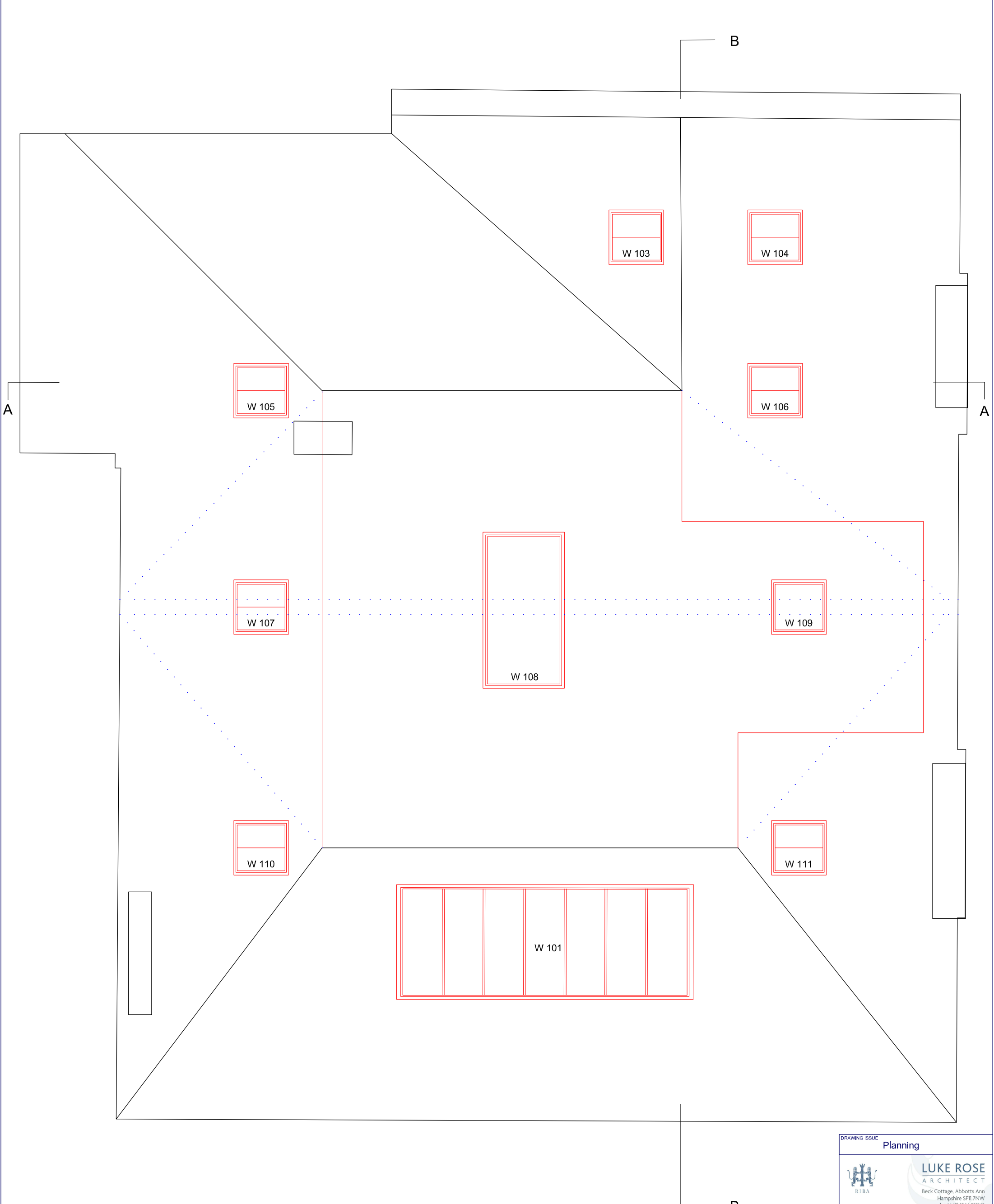
Proposed roof floor plan
