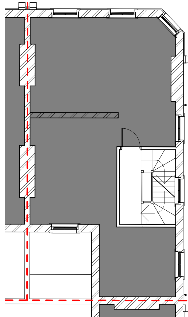
First Floor Plan Flat 1
