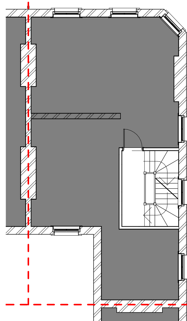
Second Floor Plan Flat 2
