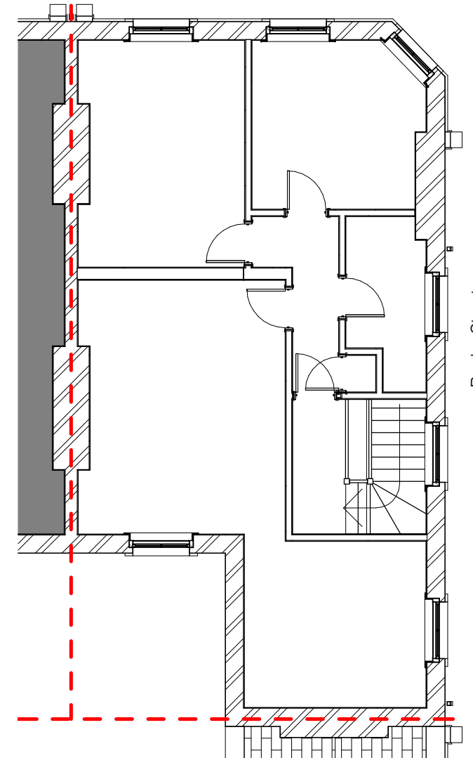
Third Floor Plan Flat 3
