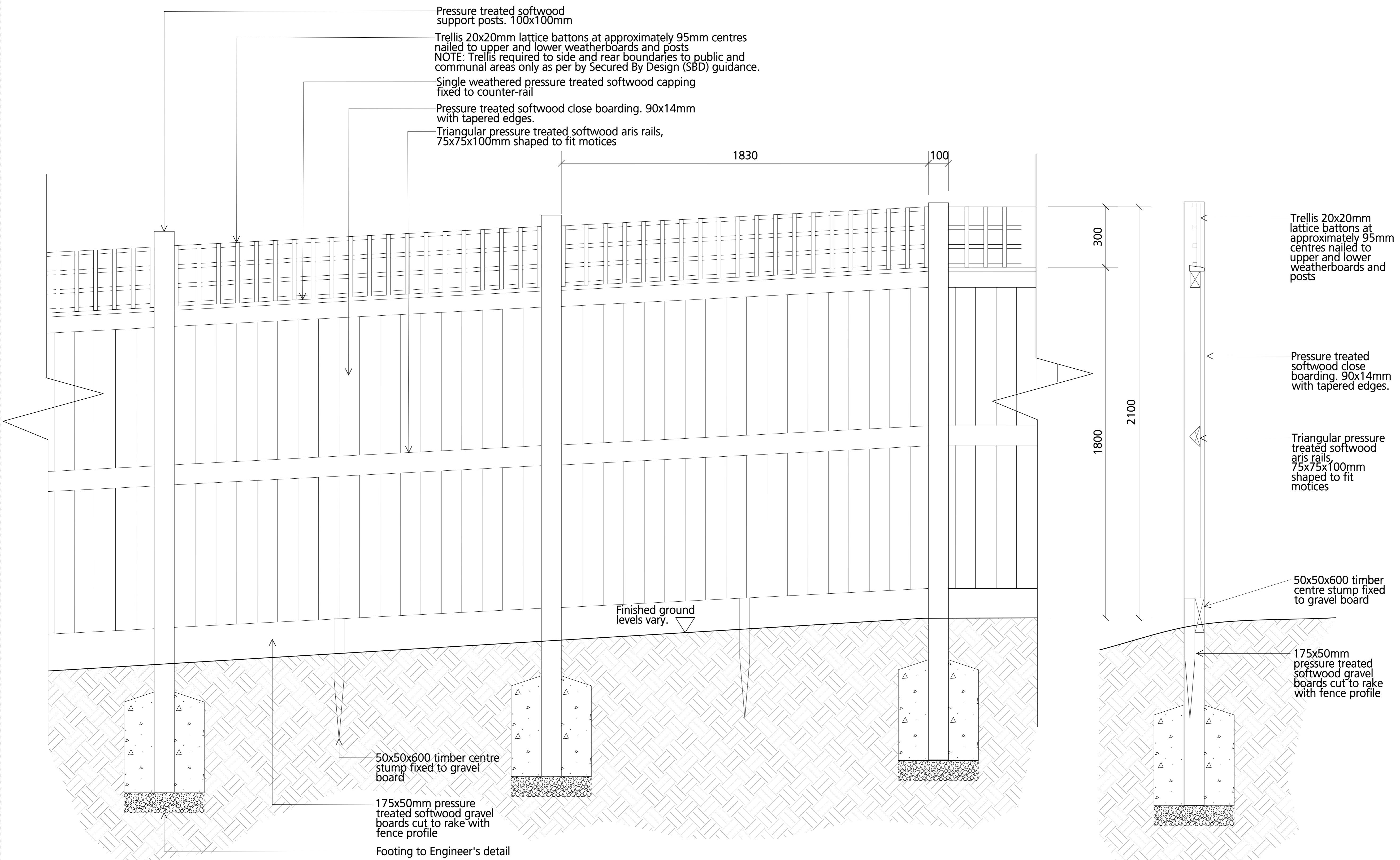
12 BOUNDARY DETAIL 9703 Timber Fence - Typical Elevation
