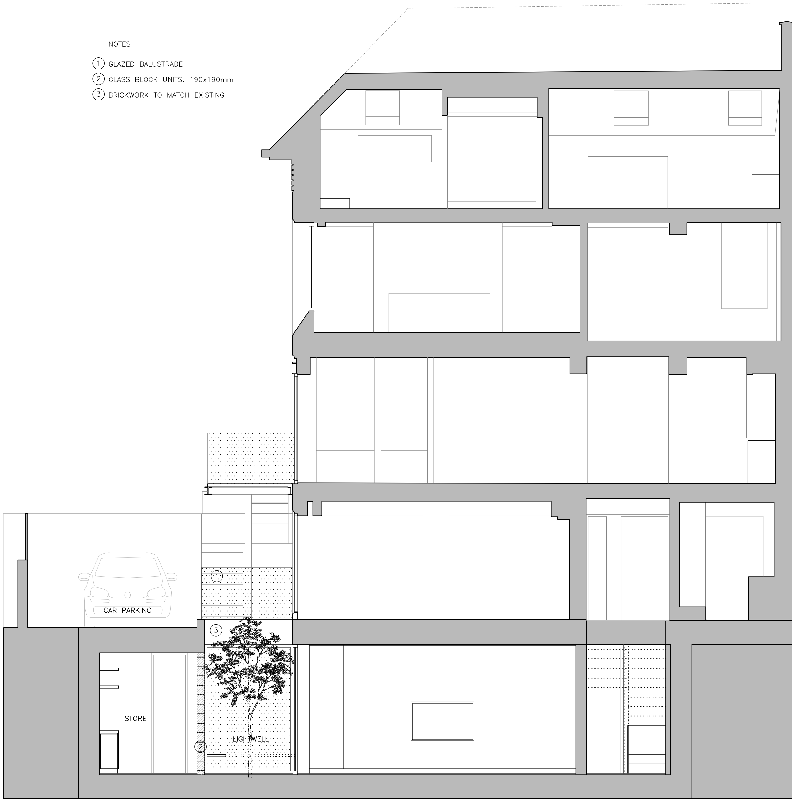
PROPOSED BUILDING SECTION C:C
