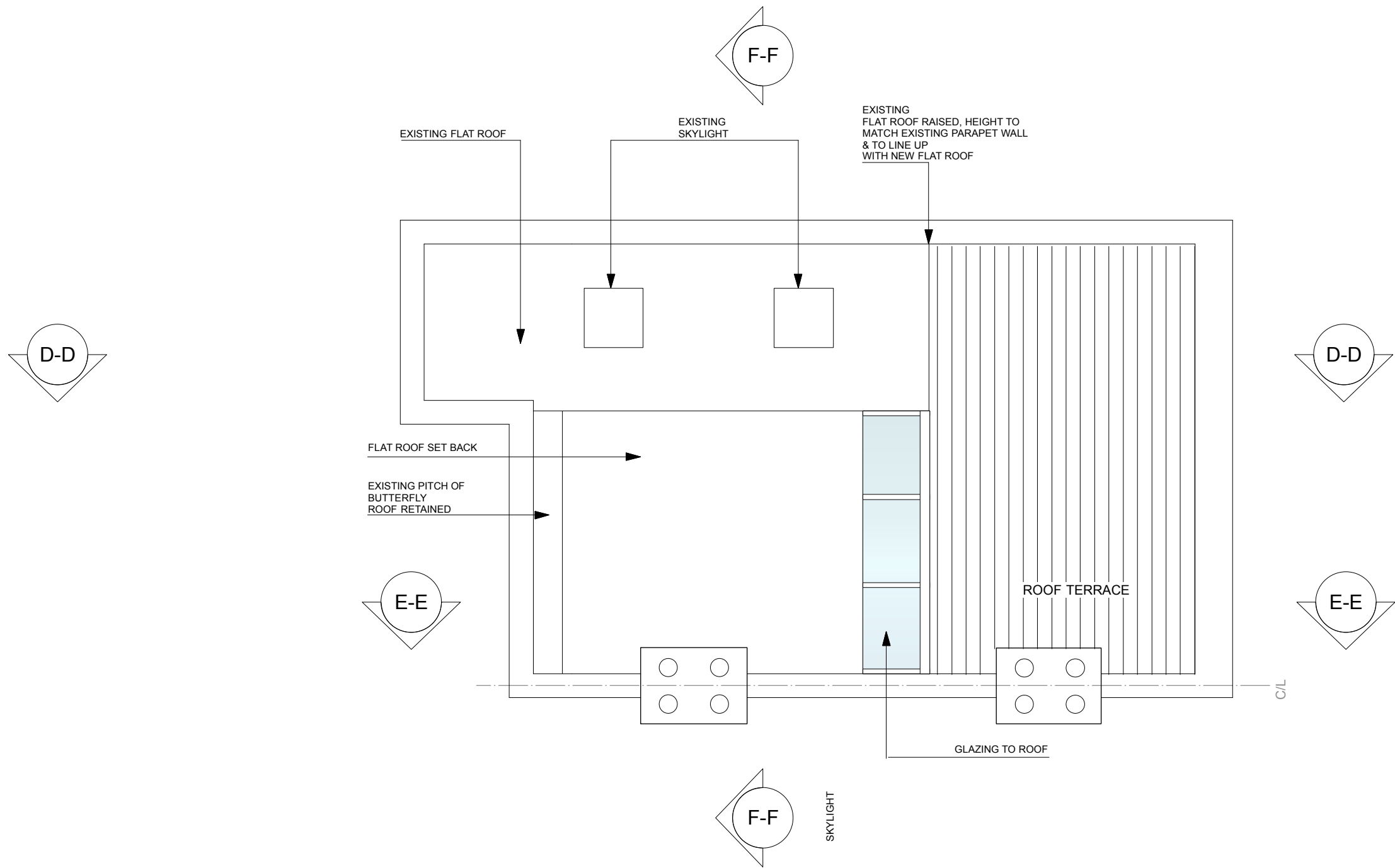
GA03 PROPOSED ROOF LAYOUT Scale: 1:50
