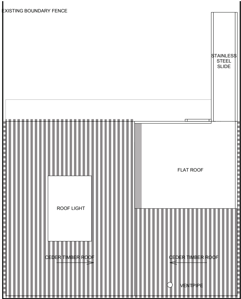
GARDEN ROOM ROOF PLAN 1:50
