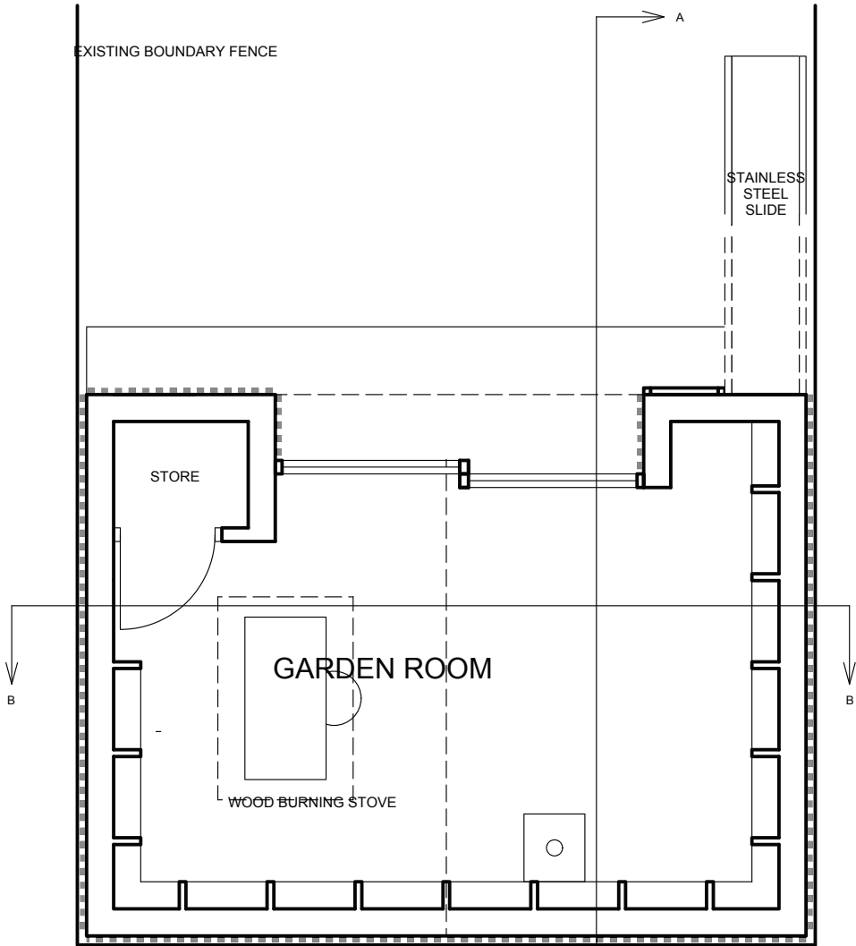
GARDEN ROOM PLAN 1:50
