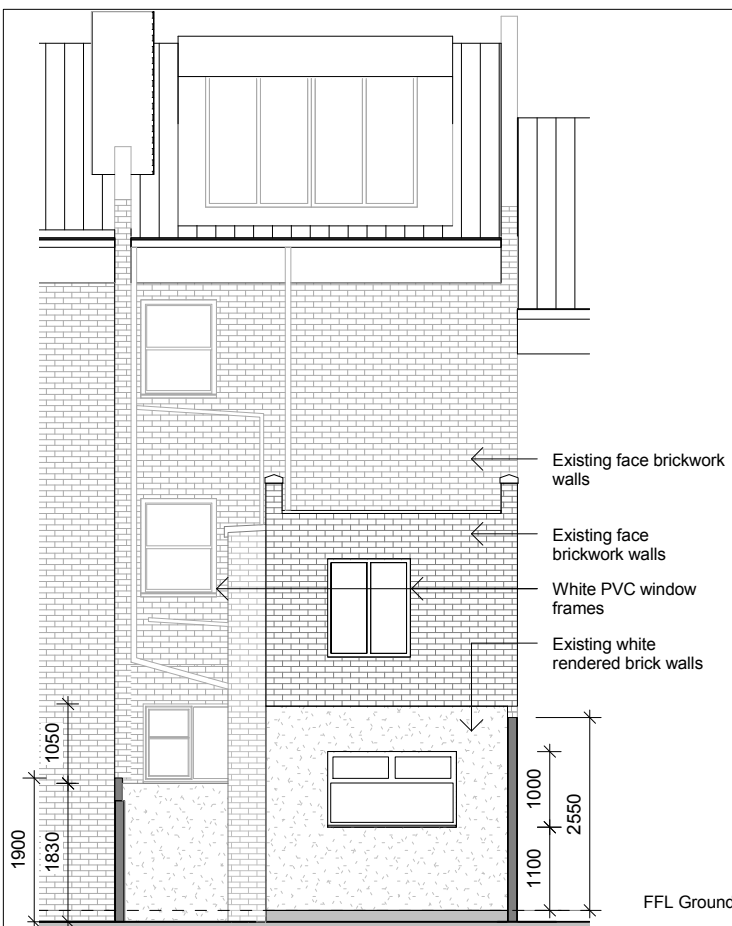
EXISTING SOUTH ELEVATION
