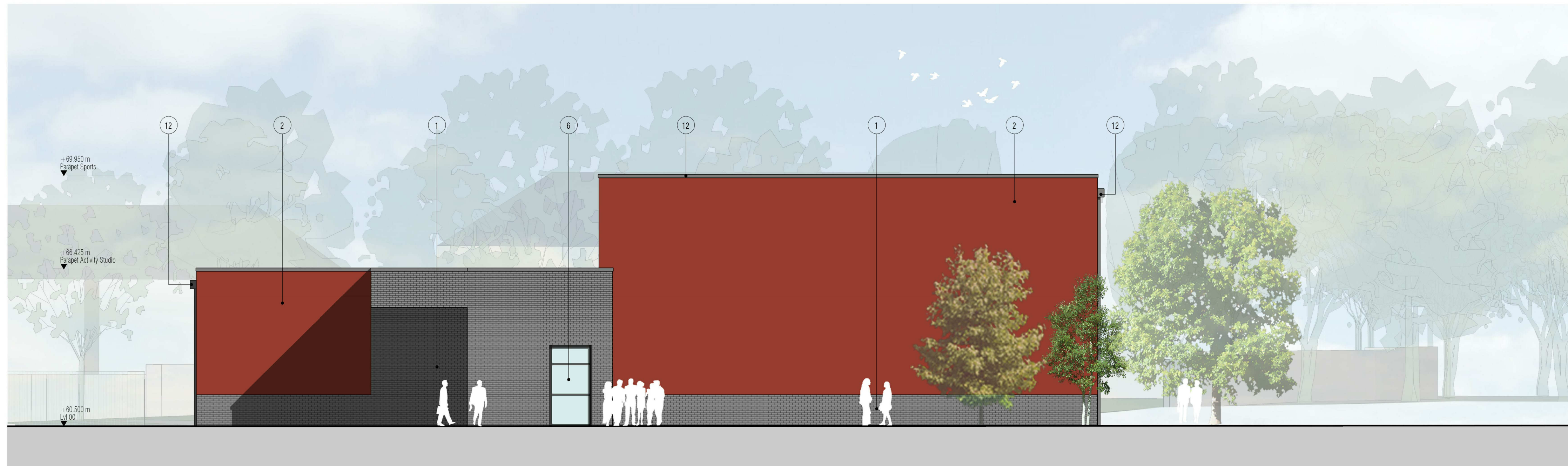
1 SOUTH ELEVATION JW-210 / 1:200
