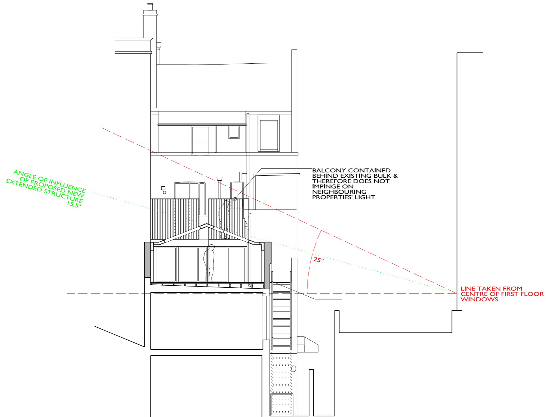
SECTION C-C'
