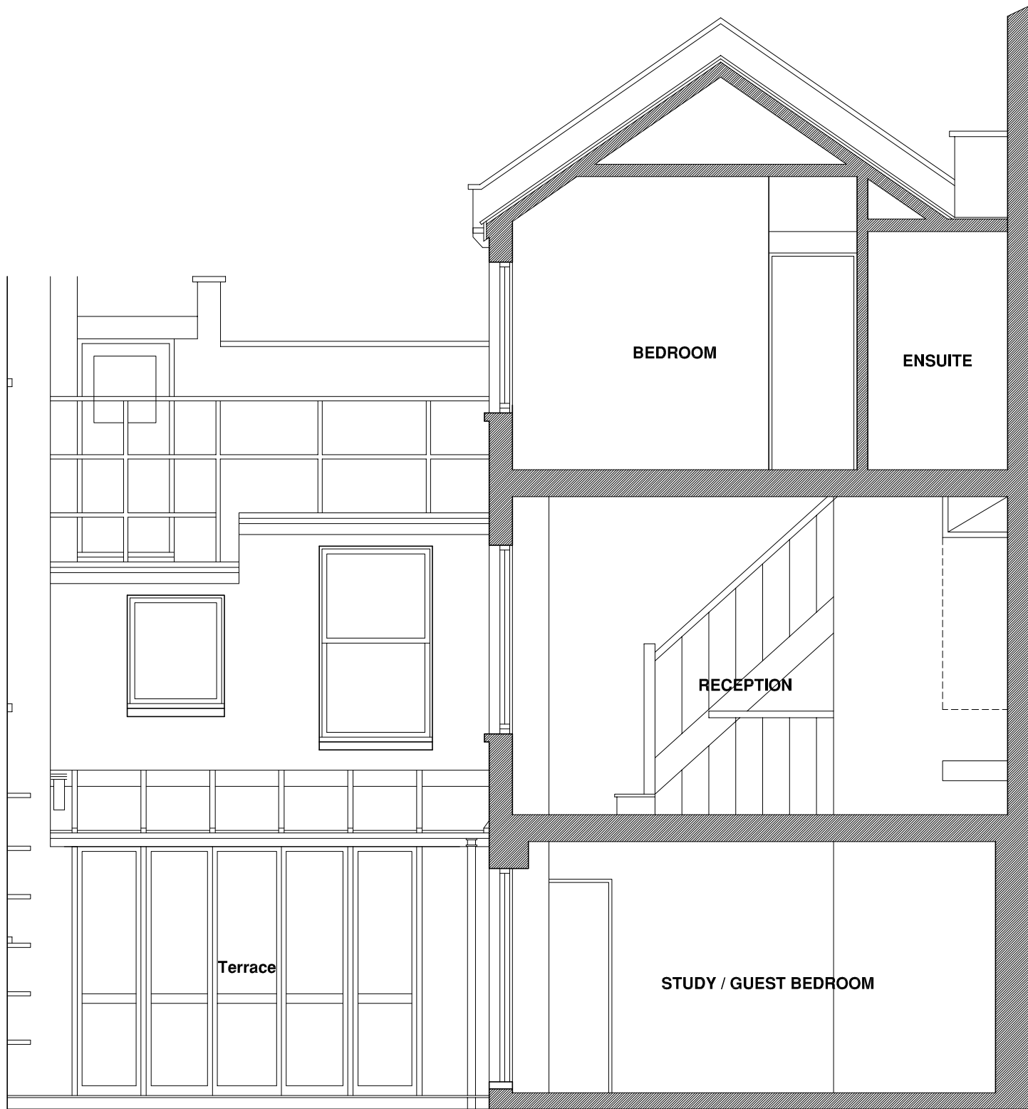
SECTIONAL ELEVATION - D
