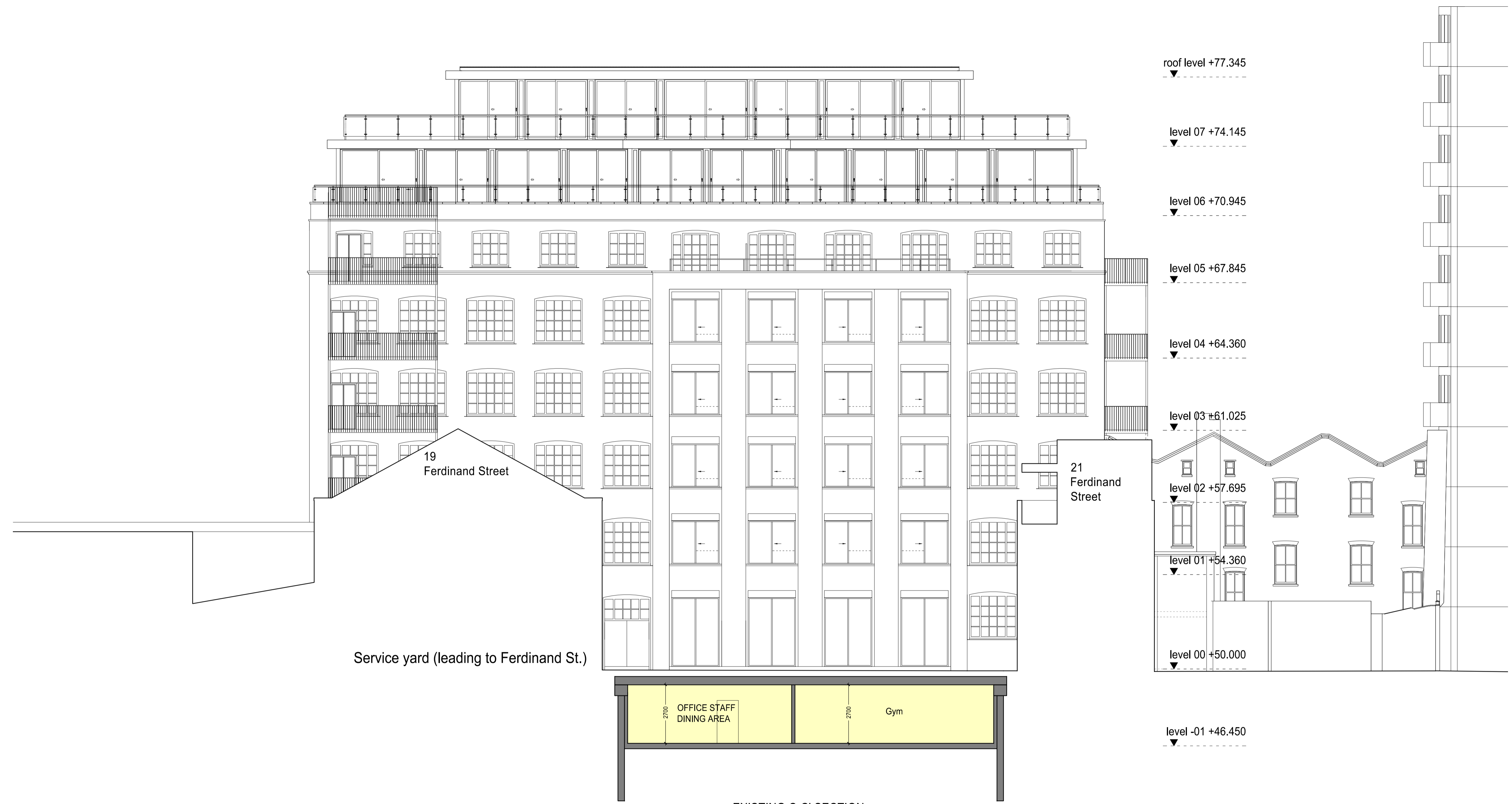
EXISTING C-C' SECTION
