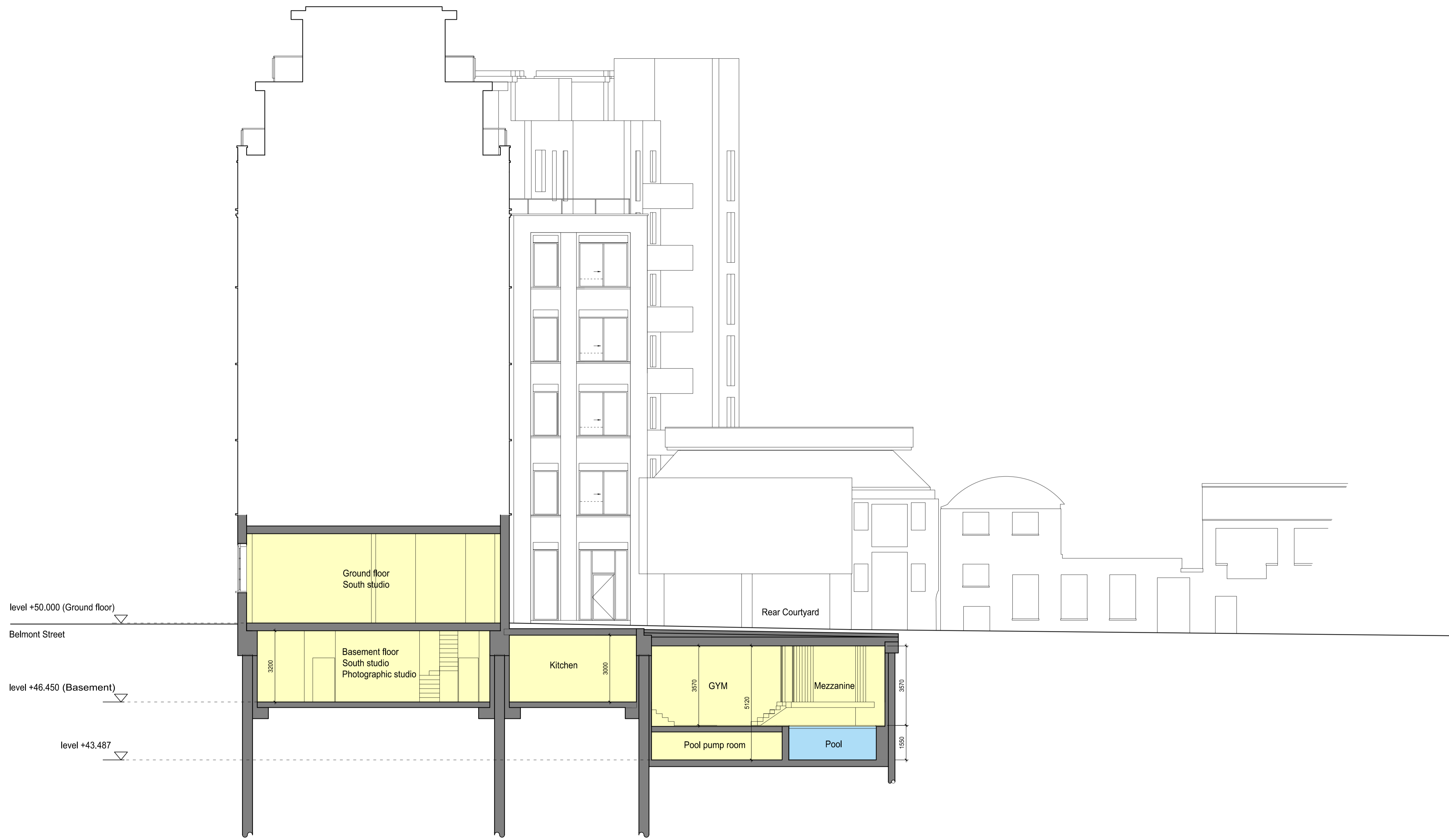
PROPOSED B-B' SECTION
