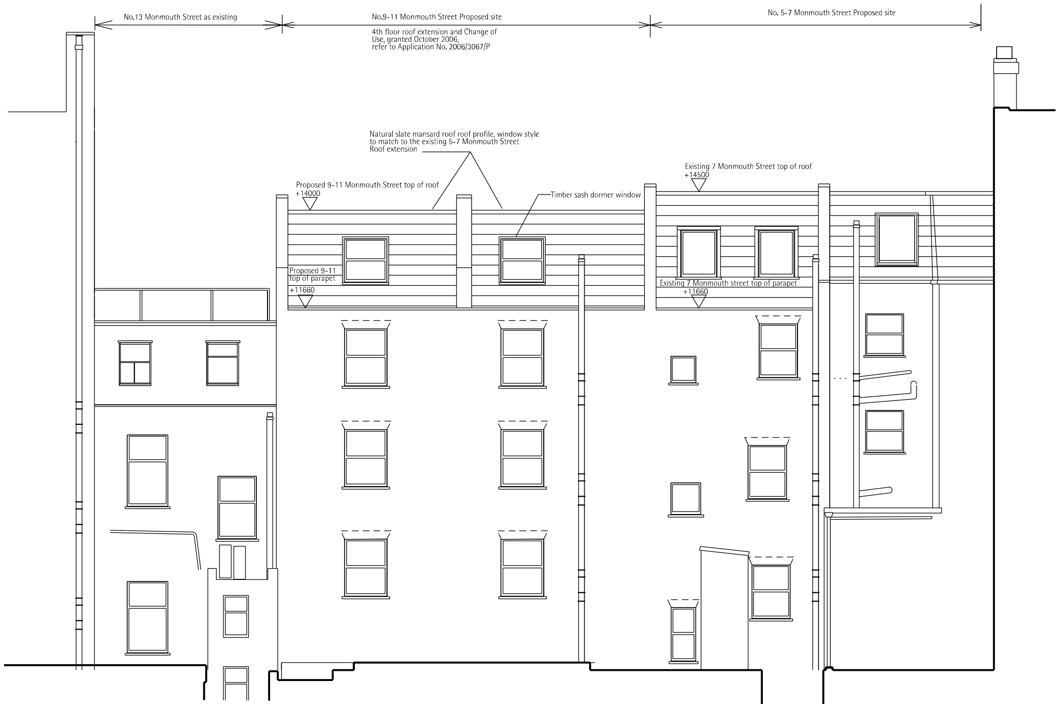
2. Proposed Rear elevation Scale 1:50@A1
