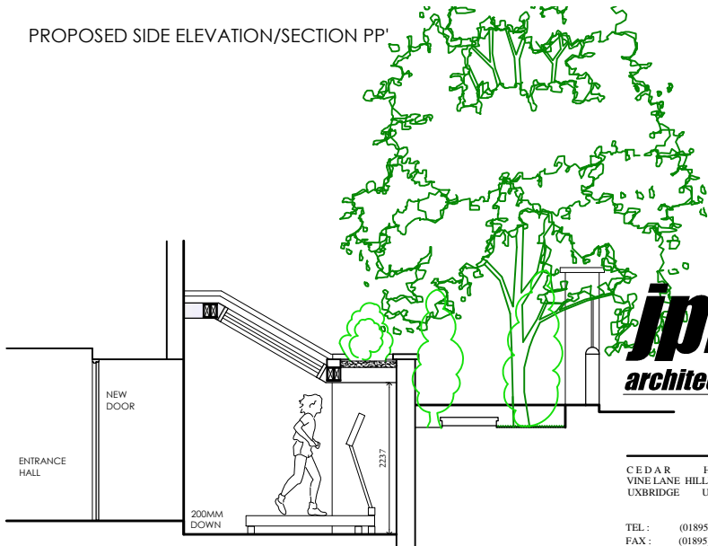
SECTION RR'
